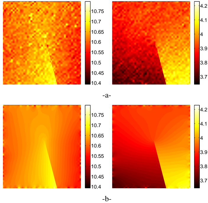
Figure 7. Vertical (left) and horizontal (right) displacement map for the SiC specimen for 16-pixel elements using: X-DIC (a), XI-DIC (b). The conversion factor is p = 1.85 \mu\text{m}/\text{pixel} .
