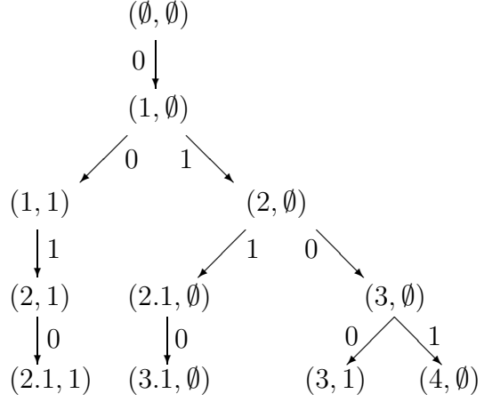
Crystal graph of \mathcal{M}[2, 0]
