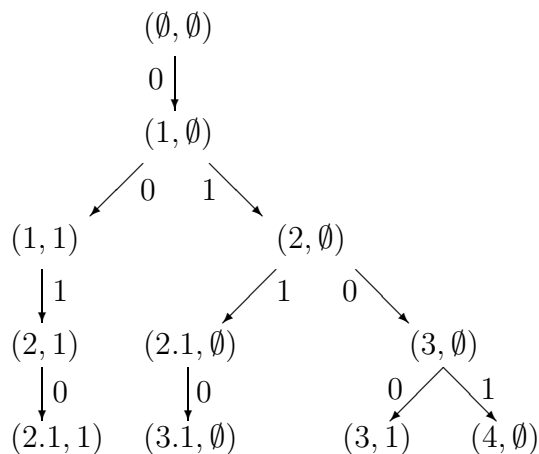
Crystal graph of \mathcal{M}[2, 0]
