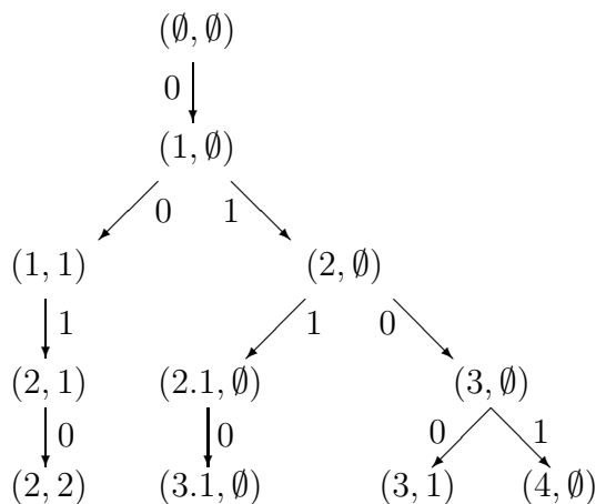
Crystal graph of \mathcal{M}[0, 0]
