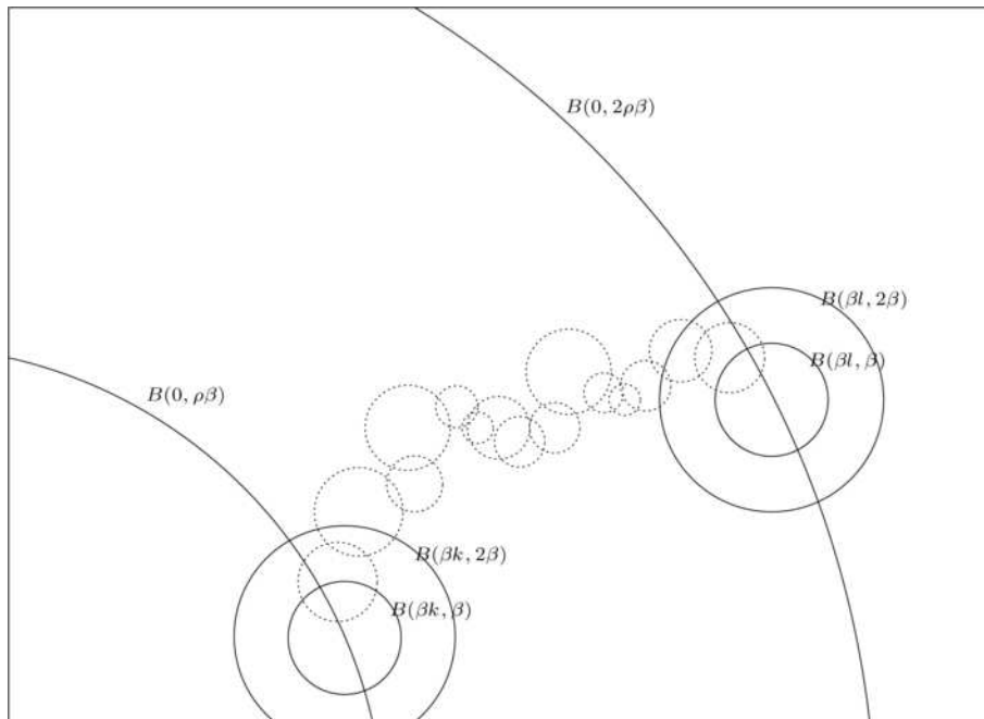
FIG. 1. Proof of (9).
