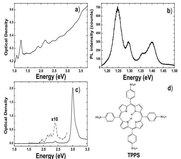
Figure 1: a) Optical absorption of CoMoCat nanotubes embedded in Sodium Dodecyl Sulfate micelles in a pH 8 Normadose buffer. b) Corresponding photoluminescence spectrum of CoMoCat nanotubes embedded in micelles (excitation energy: 2.331 eV). c) Optical absorption of TPPS in a pH 8 Normadose buffer (dashed curve: Q bands contribution rescaled for clarity). d) Chemical structure of TPPS. The phenyl groups are not in the plane of the macrocycle because of the steric hindrance.
