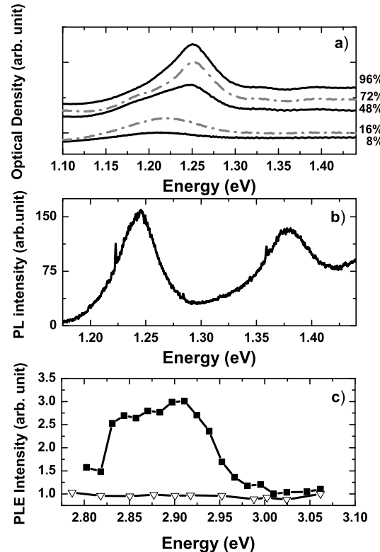
Figure 3: a) Optical density of TPPS/CoMoCat nanotubes suspension around first excitonic transition of nanotubes for different concentrations of porphyrins (from 8% to 96%). Curves have been arbitrary shifted on the Y-axis for clarity. b) Photoluminescence signal of CoMoCat nanotubes in presence of TPPS excited at 2.331 eV. c) Photoluminescence excitation spectra of a porphyrin/nanotube suspension (black squares) and of nanotubes embedded in SDS micelles (open triangles) detected at 1.246 eV.
