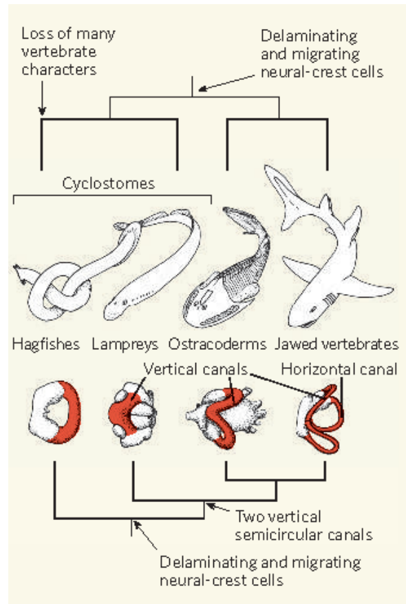
Figure 1 | The hagfish puzzle. Ota et al. 1 show that hagfishes have delaminating and migrating neural-crest cells, a feature of vertebrate head development. But it is still not clear whether hagfishes are ‘degenerate’ cyclostomes (top tree), or are ‘primitive’ and are the sister group of all other vertebrates (bottom tree). This second hypothesis is supported by many characters shared only by lampreys, jawed vertebrates and jawed-vertebrate precursors, the 480–365-million-year-old jawless ostracoderms. Notably, there are differences in the canals (red) of the inner ear (labyrinth): the hagfish labyrinth possesses a single semicircular canal for balance, whereas all other vertebrates have at least two, vertical, canals.
