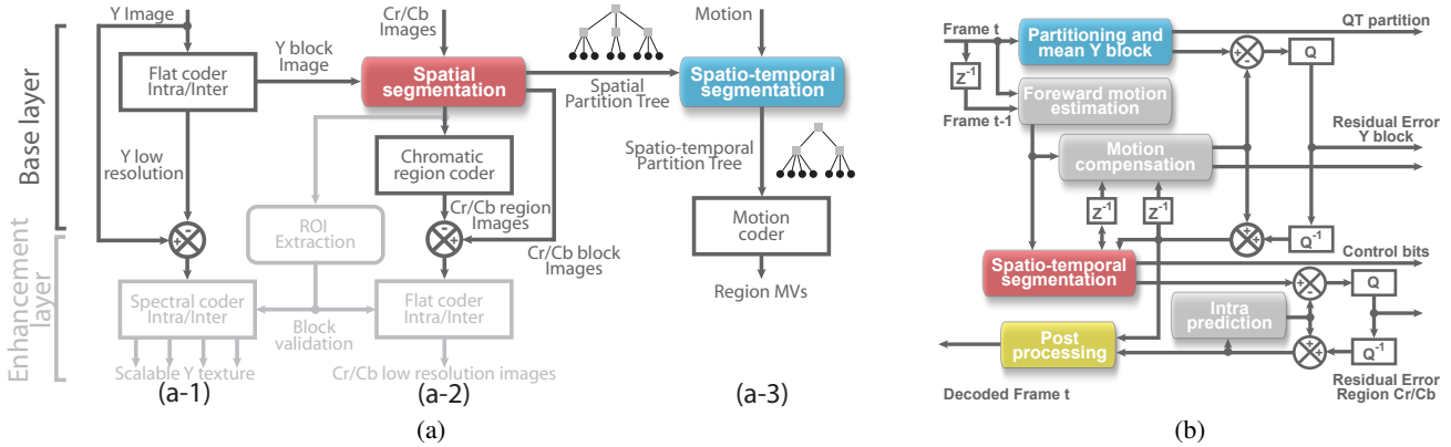
Figure 1: (a-1) Luminance Y image coder. (a-2) Region-based chromatic component (Cr/Cb) representation and compression. (a-3) Region-based motion representation and compression. (b) Simplified description of the LAR video encoder with the output stream
