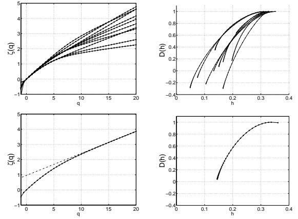
Fig. 2. Linearisation effect on experimental turbulence (velocity) data. Estimated \zeta(q) (left column) and corresponding D(h) (right column) for 10 runs (top row) and averaged over 69 runs (bottom row), with n = 2^{20} and \simeq 60 integral scales per run.
