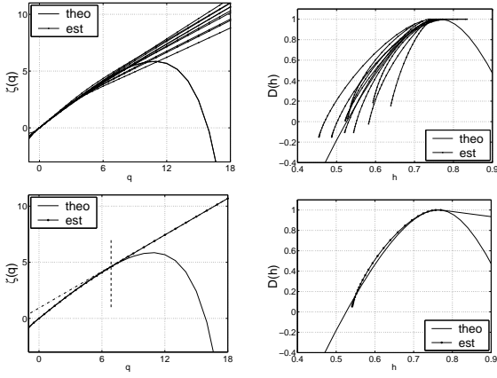
Fig. 1. Linearisation effect on synthetic data. Theoretical and estimated \zeta(q) (left column) and corresponding D(h) (right column), for 10 replications (top row) and averaged over 1000 replications (bottom row). FBM(MT) built on CMC cascades, with n = 2^{19} and 2^4 integral scales.
