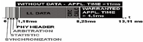
Fig.2. Le protocole AwareCON
