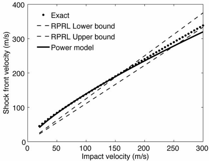
Figure 15. Comparison of models in terms of shock front velocity vs. impact velocity
