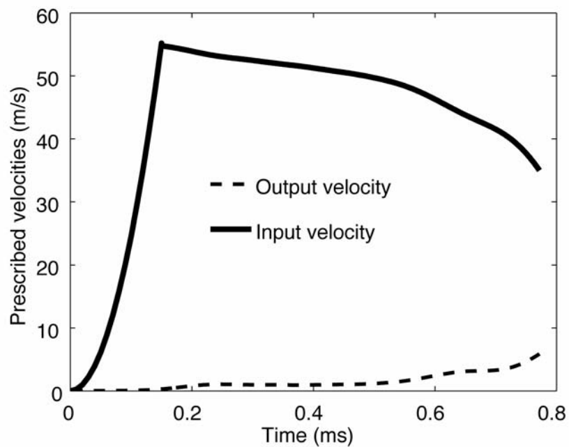
Figure 4. Input and output prescribed velocities for the moving rigid walls (config. 1)
