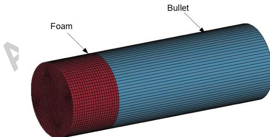
Figure 6. Foam and projectile against a moving rigid wall (config. 2)
