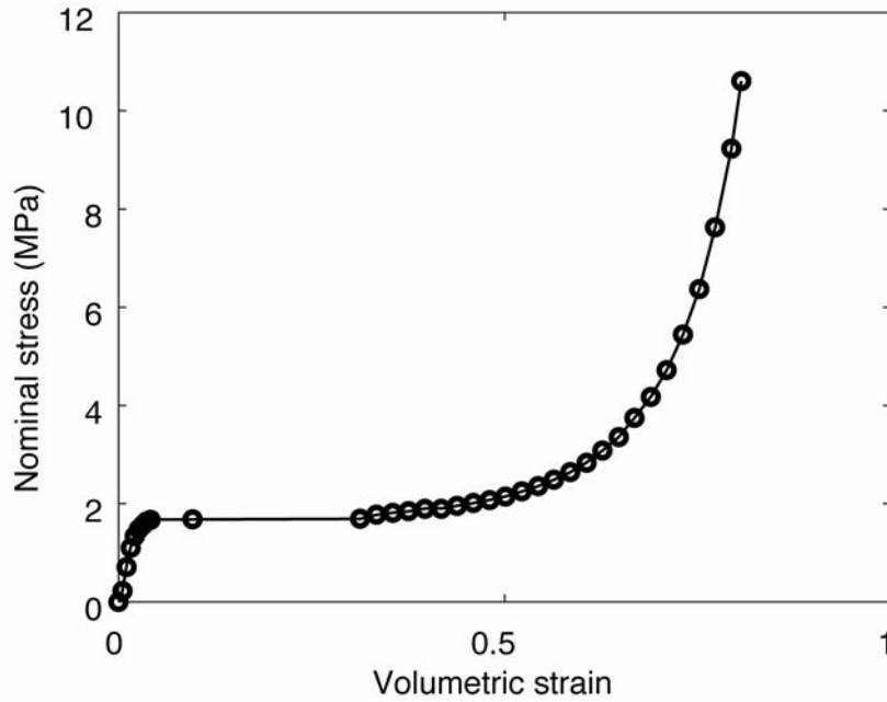
Figure 2. Input flow stress-volumetric strain relation for Alporas foam
