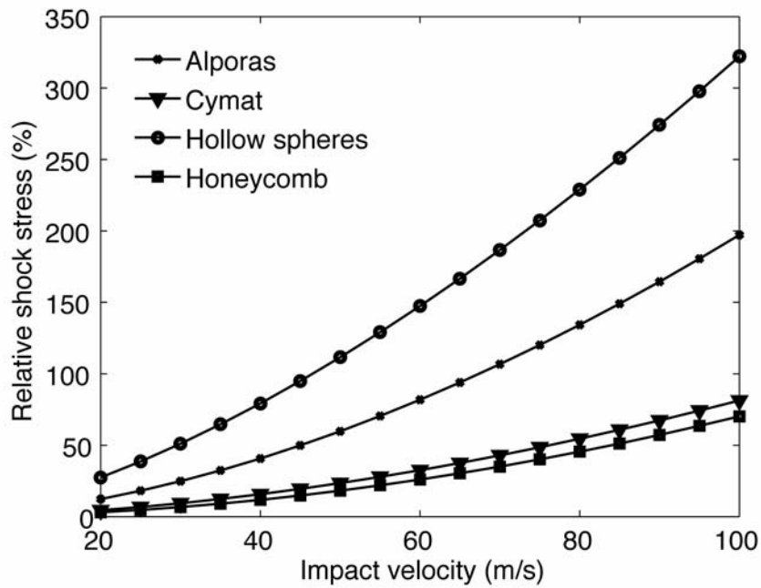
Figure 16 Shock enhancement effect for the four studied materials
