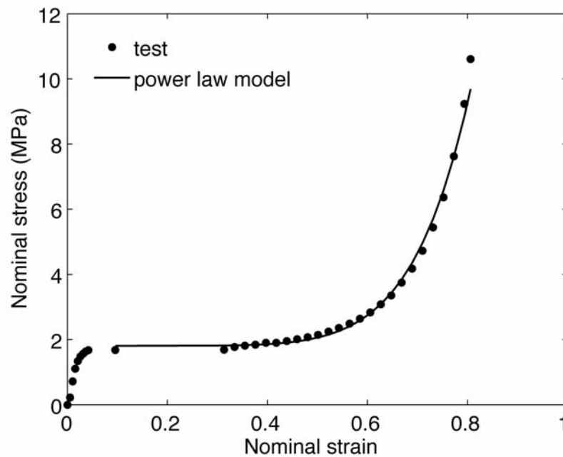
Figure 14. Power law model identification for Alporas foam
