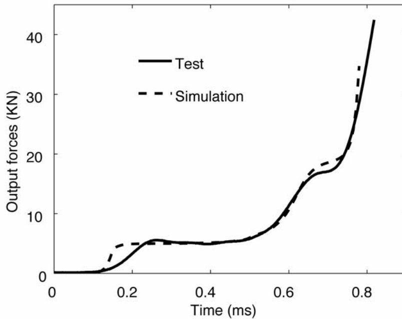
Figure 5. Comparison between simulated and measured force / time histories (config. 1)
