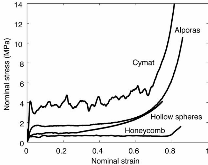
Figure 11. Typical quasi-static behaviour of tested materials
