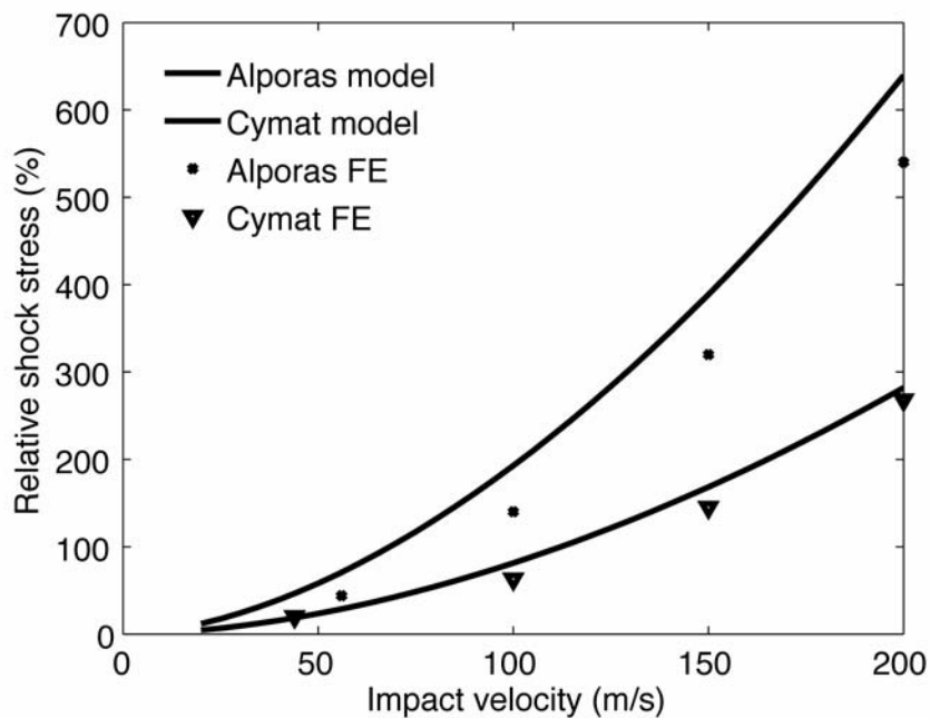
Figure 17 Comparison between FEM analyses and power model for the prediction of the relative shock stress vs. impact velocity.
