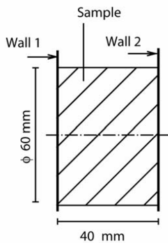
Figure 3. Boundary conditions for simulating test configuration 1
