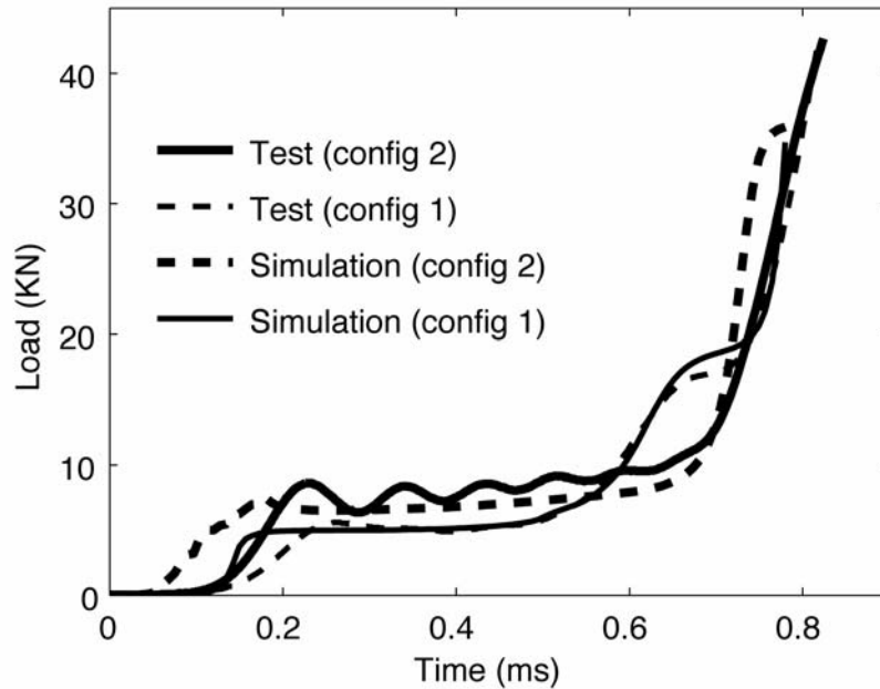
Figure 9. Comparison between experimental and simulated force histories
