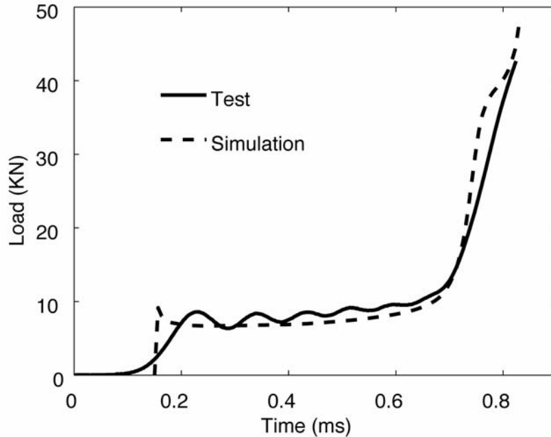
Figure 7. Comparison between simulated and measured force / time histories (config. 2)
