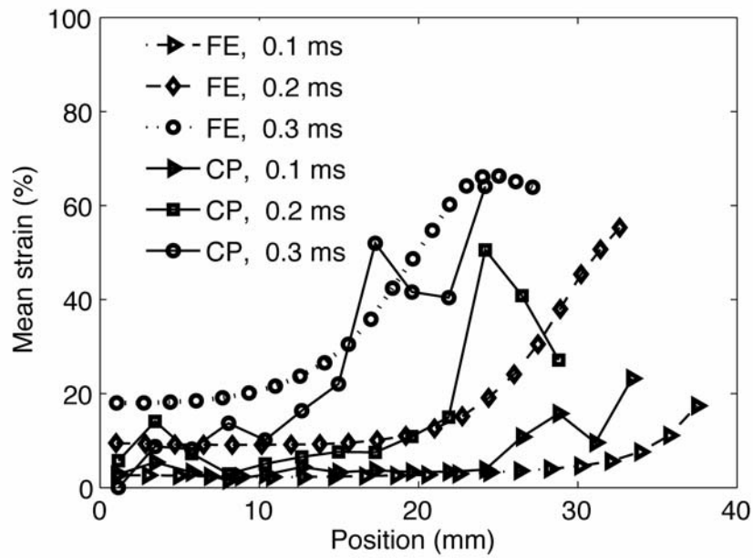
Figure 10. Comparison of simulated (FE) and measured (CP) strain discontinuity profiles
