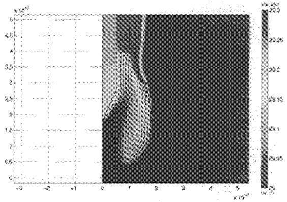
Figure 2: Velocity field and temperature contour lines in the droplet obtained with a 20 °C temperature difference between the heated rod and the cold plate.
