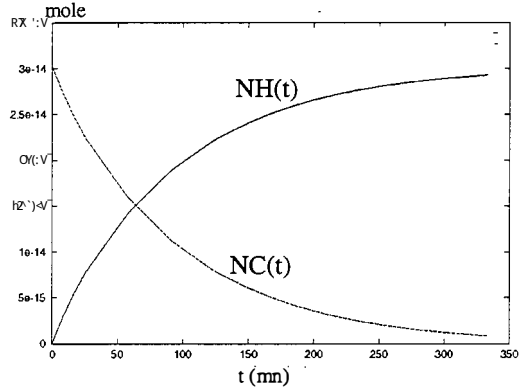
Figure 5: Binding kinetics NH(t) in the case (b).
