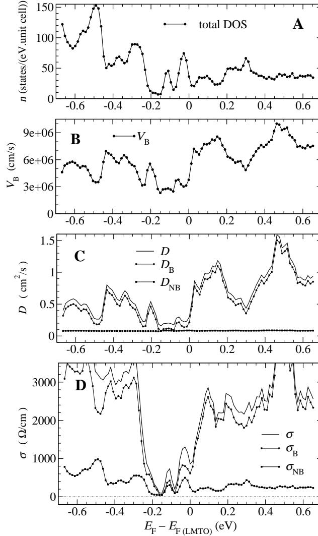
Figure 2. (A) LMTO total DOS n , (B) Boltzmann velocity V_B , (C) diffusivity D = D_B + D_{NB} , and (D) conductivity \sigma = \sigma_B + \sigma_{NB} , in the cubic approximant \alpha -Al 69.6 Si 13.0 Mn 17.4 . Points are the calculated values and lines are guides for the eyes. D and \sigma are calculated for \tau = 1.5 \times 10^{-14} s.
