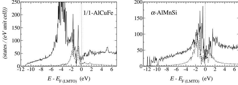
Figure 1. Ab-initio LMTO DOS in \alpha -Al 69.6 Si 13.0 Mn 17.4 and Al 78 Cu 48 Fe 13 1/1-cubic approximant: (line) total DOS and (dashed line) local TM DOS (TM = Mn or Fe).
