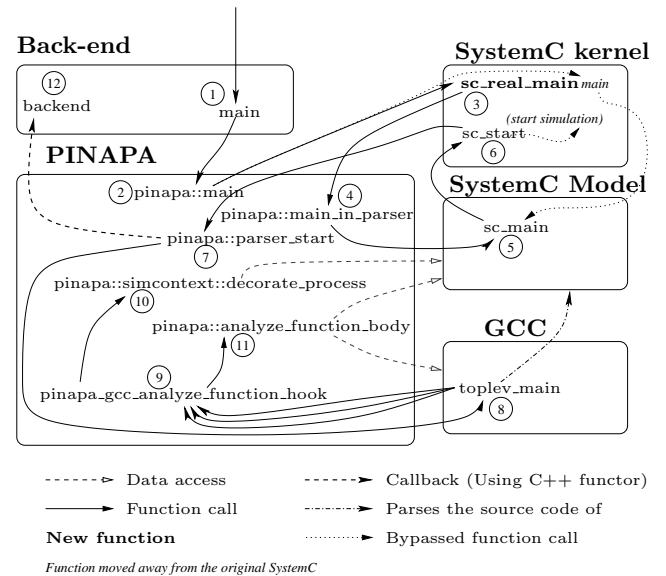
Figure 6: Architecture of PINAPA
