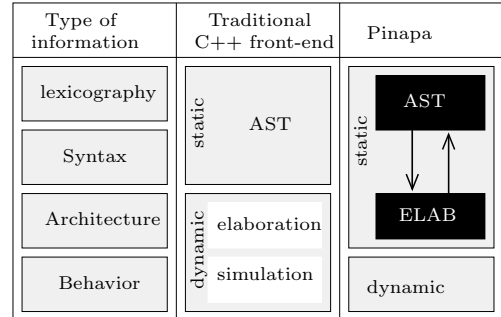
Figure 3: Static and Dynamic information in a SystemC program
