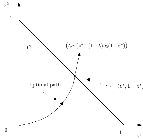
Figure 4: Optimal deadlock point and path, Case 1 with \lambda < 1/2 , g_1(0) = g_2(0) = 0
