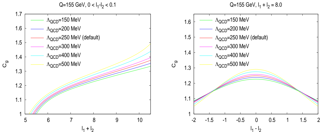
Figure 15: dependence of the gluonic 2-particle correlation function C_g on \Lambda_{QCD} .
