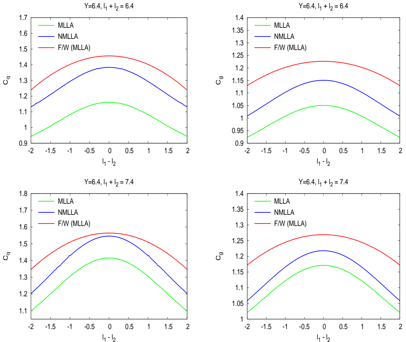
Figure 14: 2-particle correlations for a quark jet (left) and a gluon jet (right) as a function of \ell_1 - \ell_2 ; MLLA, NMLLA and Fong-Webber prediction.
