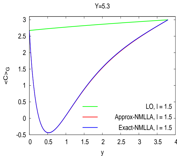
Figure 19: Approximate (used in the core of the paper) and exact color currents for a gluon jet.
