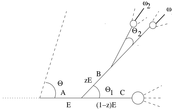
Figure 11: 2-particle correlations inside a jet
