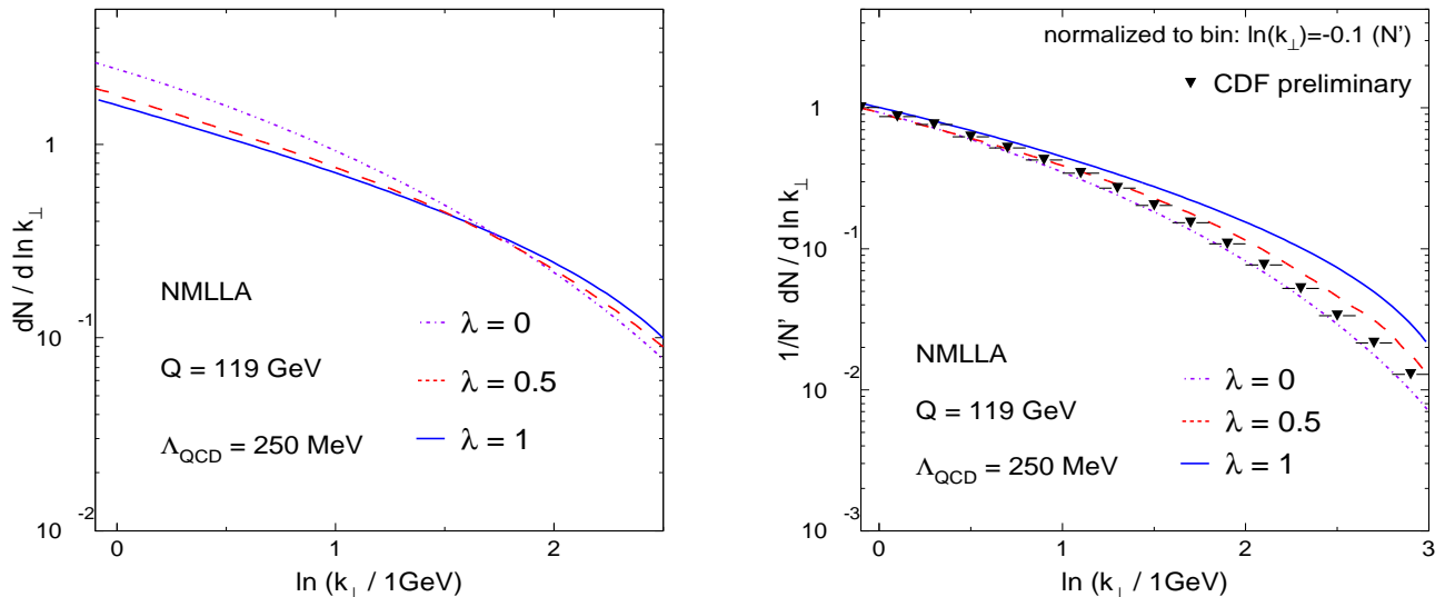
Figure 10: Absolute (left) and normalized (right) inclusive k_{\perp} -distribution beyond the limiting spectrum approximation at NMLLA in a jet of hardness Q = 119 \text{ GeV} .
