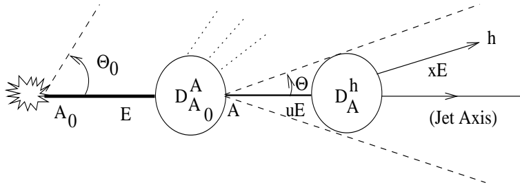
Figure 2: Inclusive production of hadron h at an angle \Theta inside a high energy jet of total opening angle \Theta_0 .
