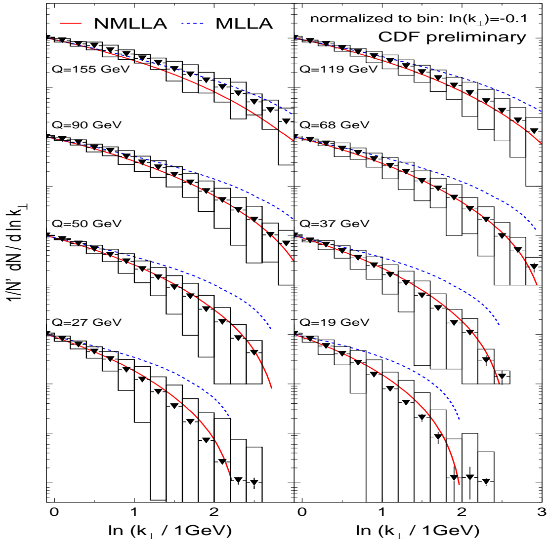
Figure 5: CDF preliminary results on hadronic single-inclusive k_{\perp} -distributions, compared with MLLA (dashed lines) and NMLLA (solid lines) calculations at the limiting spectrum; the boxes are the systematic errors (their lower limits are cut at large k_{\perp} for the sake of clarity)
