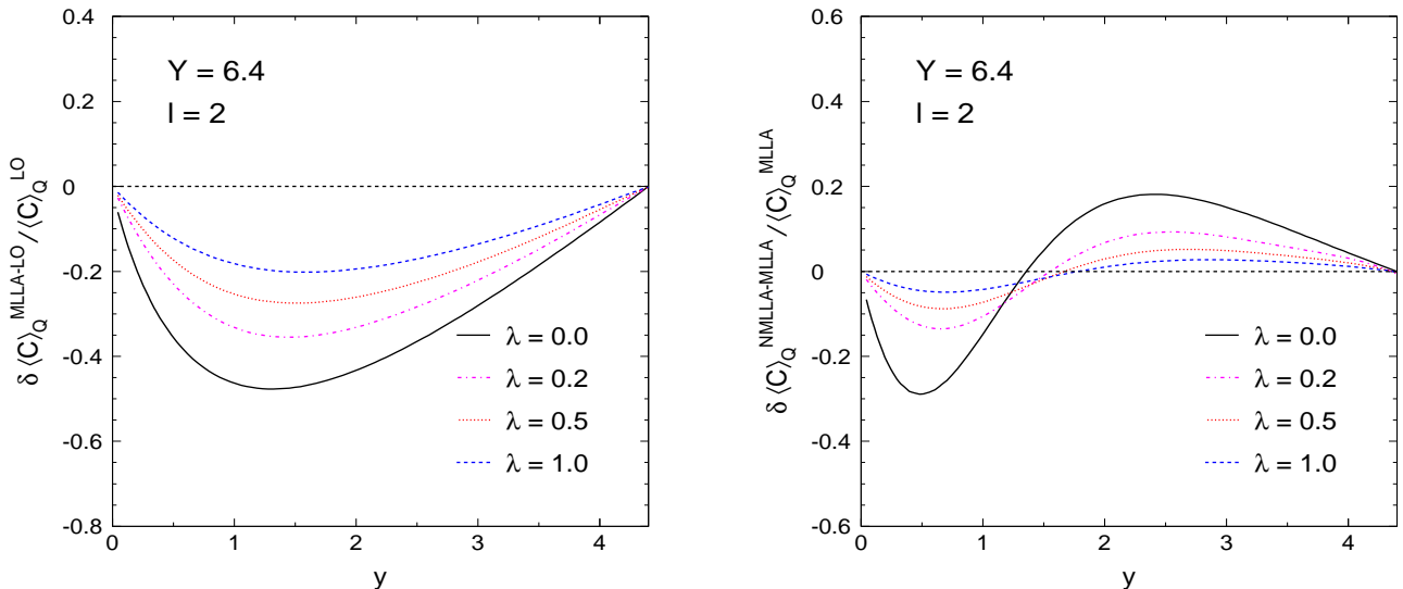
Figure 8: MLLA (left) and NMLLA (right) normalized corrections to the LO and MLLA color currents, respectively, for different values of \lambda .
