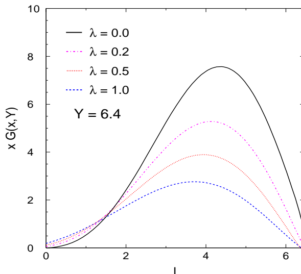
Figure 7: Inclusive spectrum for a gluon jet ( Y_{\Theta_0} = 6.4 ) for different values of \lambda .
