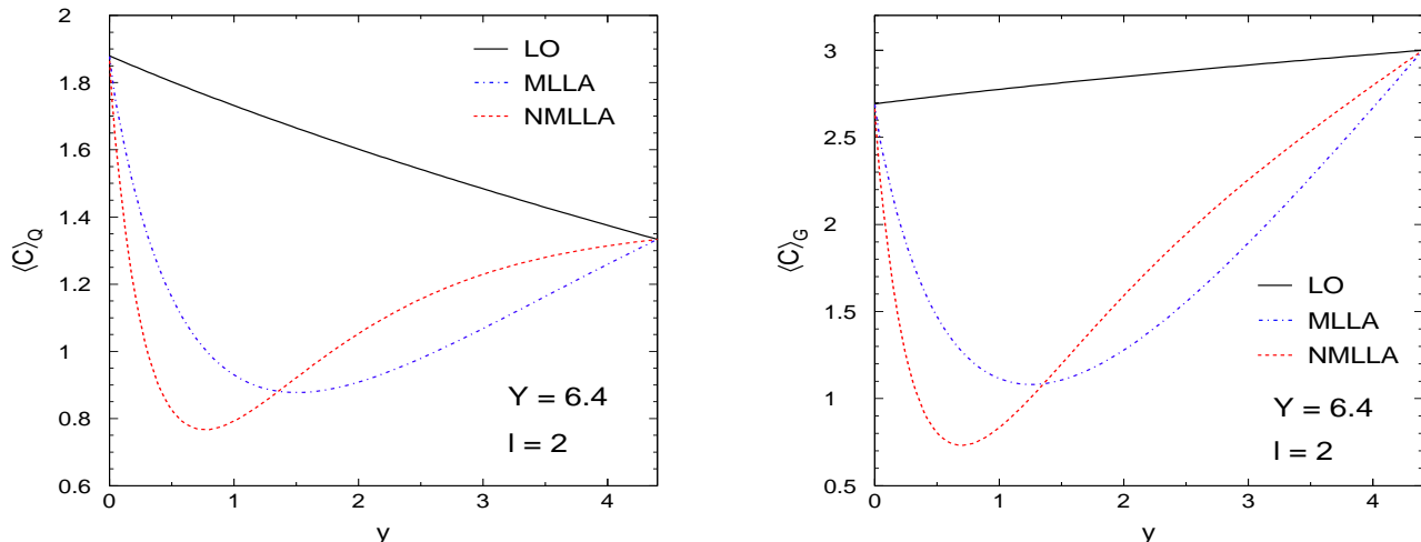
Figure 3: Color currents at LO (solid lines), MLLA (dash-dotted), and NMLLA (dashed) for a quark (left) and gluon jet (right) with Y_{\Theta_0} = 6.4 and \ell = 2 .
