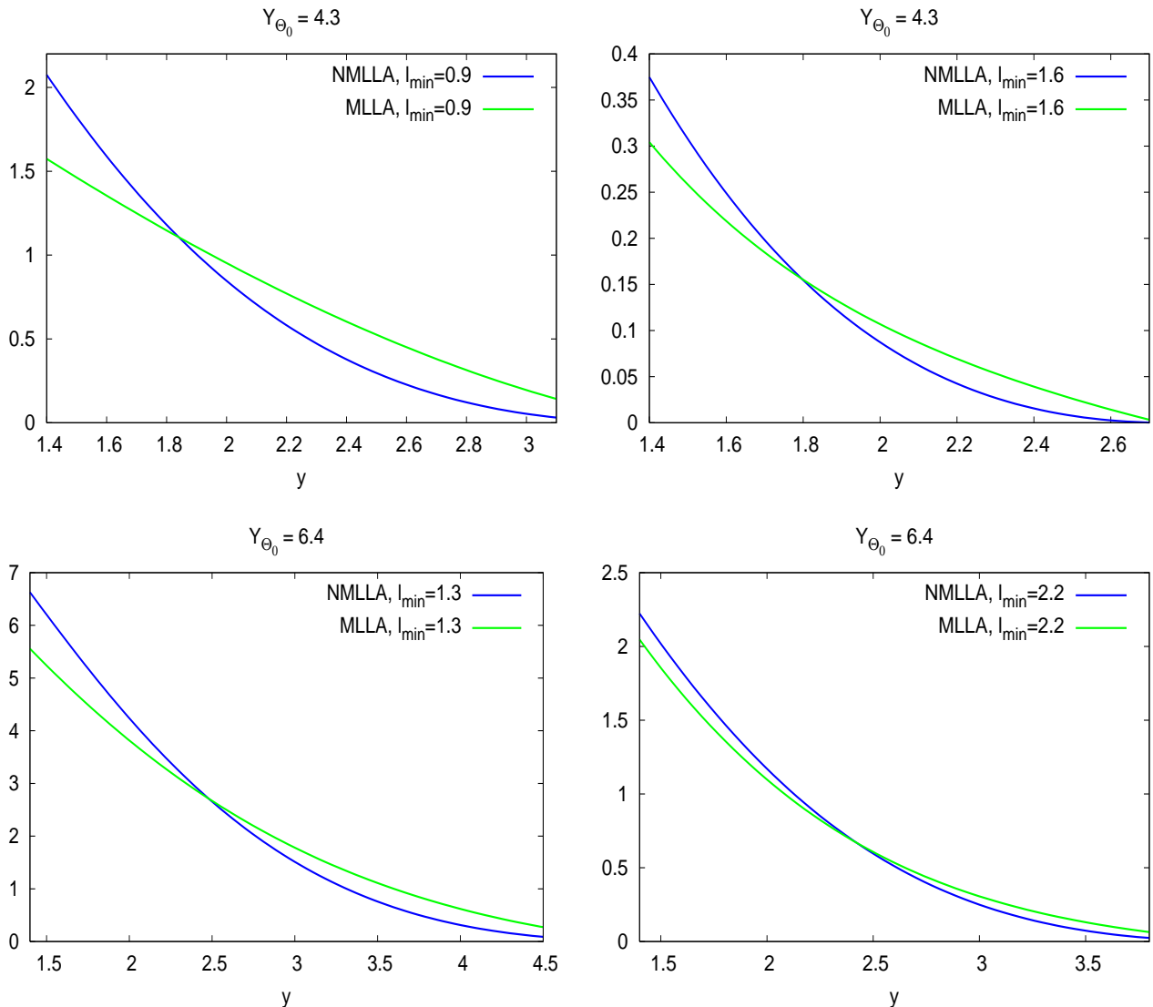
Figure 4: MLLA (green) and NMLLA (blue) inclusive y -distributions for a quark (left) and a gluon jet (right) with Y_{\Theta_0} = 4.3 ( Q = 19 GeV) and Y_{\Theta_0} = 6.4 ( Q = 155 GeV).
