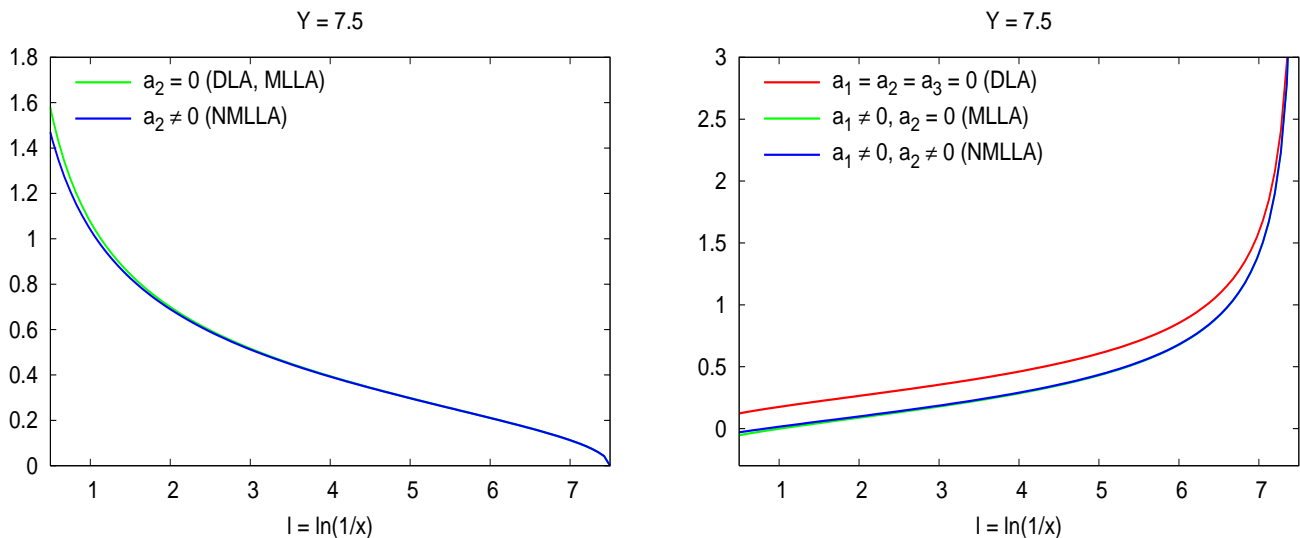
Figure 17: Logarithmic derivatives \psi_\ell (left) and \psi_y (right) of the inclusive spectrum G(\ell, Y_{\Theta_0}) at Y_{\Theta_0} = 7.5 .
