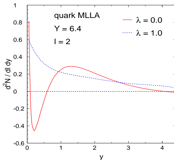
Figure 9: MLLA double differential distribution for a quark jet Y_{\Theta_0} = 6.4 computed at \lambda = 0 (solid line) and \lambda = 1 (dashed line).
