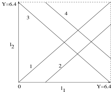
Figure 13: Positions in (\ell_1, \ell_2) space of Figs. 12 and 14.
