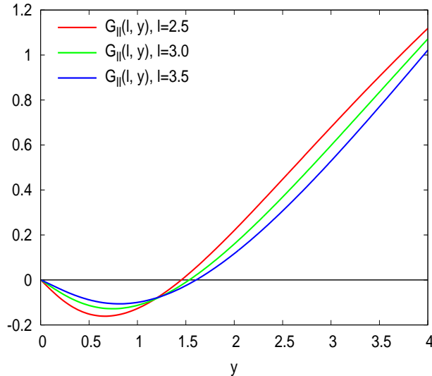
Figure 18: Second derivative of the single inclusive spectrum as a function of y at Y_{\Theta_0} = 7.5 .
