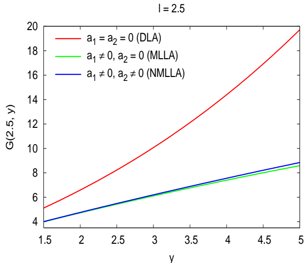
Figure 16: Single inclusive spectrum at fixed \alpha_s as a function of y at Y_{\Theta_0} = 7.5 and \ell = 2.5 .
