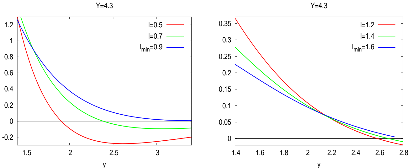
Figure 20: \frac{d^2N}{d\ell dy} for a gluon jet (left) and a quark jet (right) as a function of y for three values of \ell .
