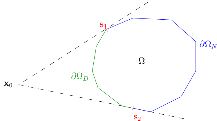
Figure 1: a convex polygonal domain \Omega with a non-empty interface \Gamma = \{\mathbf{s}_1, \mathbf{s}_2\} .
