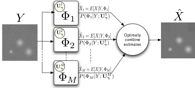
Fig. 1. The flowchart of Bayesian combined denoising.
