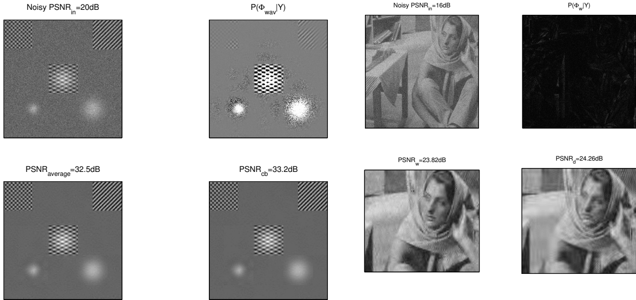
Fig. 2. Illustration on a synthetic example (texture+gaussian image with \text{PSNR}_{in} = 20\text{dB} ). From top to bottom and left to right: noisy, posterior probability map of the wavelet transform, combined estimate by averaging, optimally combined estimate.
