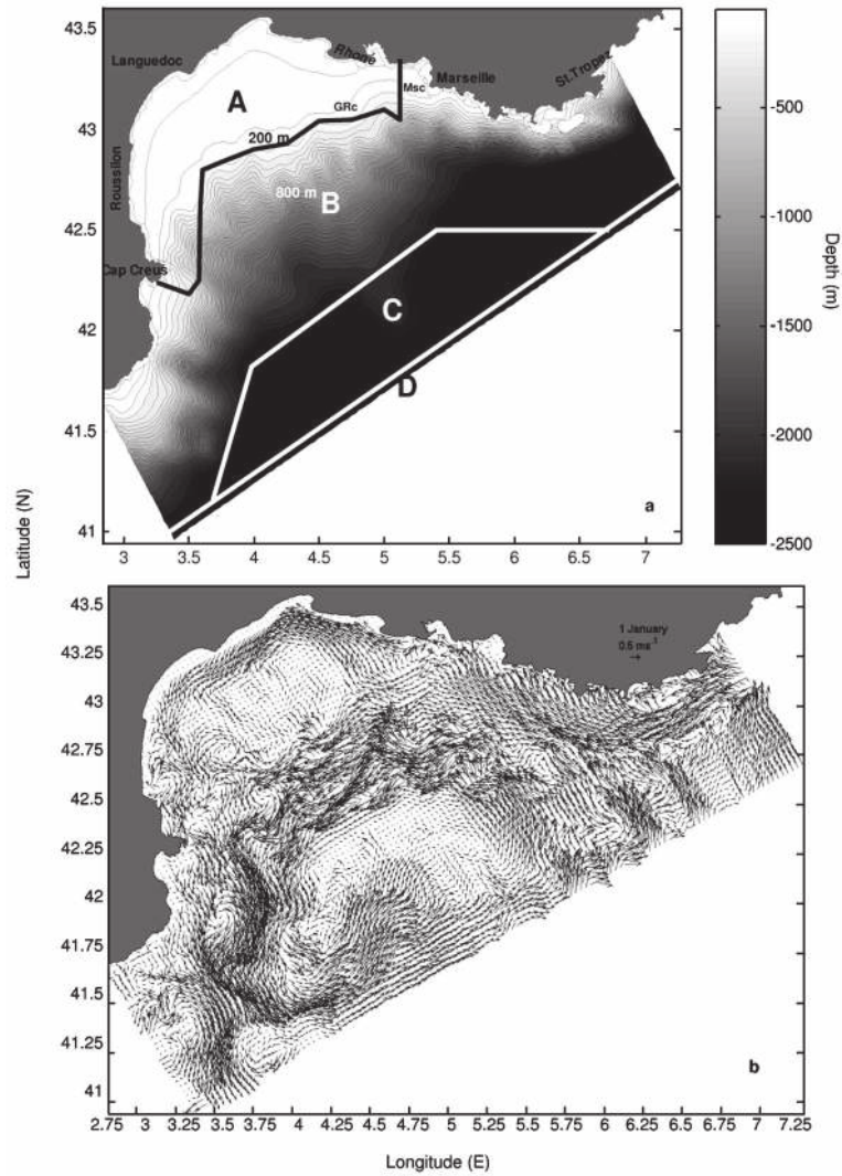
Fig. 1. – a) The modelled domain divided into four sectors and the corresponding bathymetry (interval isolines 50 m); b) the cyclonic structure of the large-scale circulation and the north-western intrusion of the NMC in the GoL visible in the horizontal velocity field (at 20 m depth) on January 1st.
