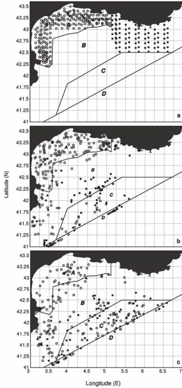
Fig. 2. – The evolution of particle distribution released from sectors A ( \circ ) and B ( \bullet ) at a) initial time step; b) after one month from the release; c) after two months from the launch. For graphical purposes only a subset of 300 particles is shown.
