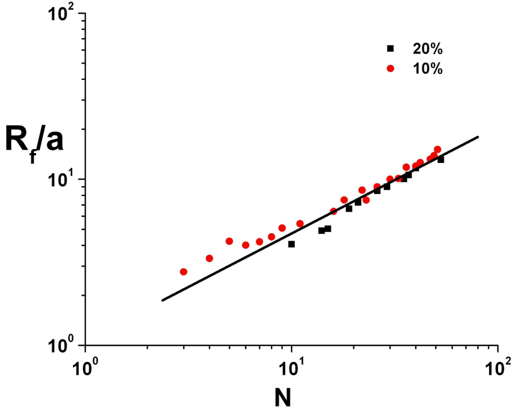
FIG. 6: Color online. Plot of \frac{R_f}{a} as a function of N to determine the fractal dimension D . Two concentrations are used: 10% and 20%. There are noticeable differences at low values of N but there is an increased accuracy for large N , where the two concentrations give rise to the same slope. D = 1.47 .
