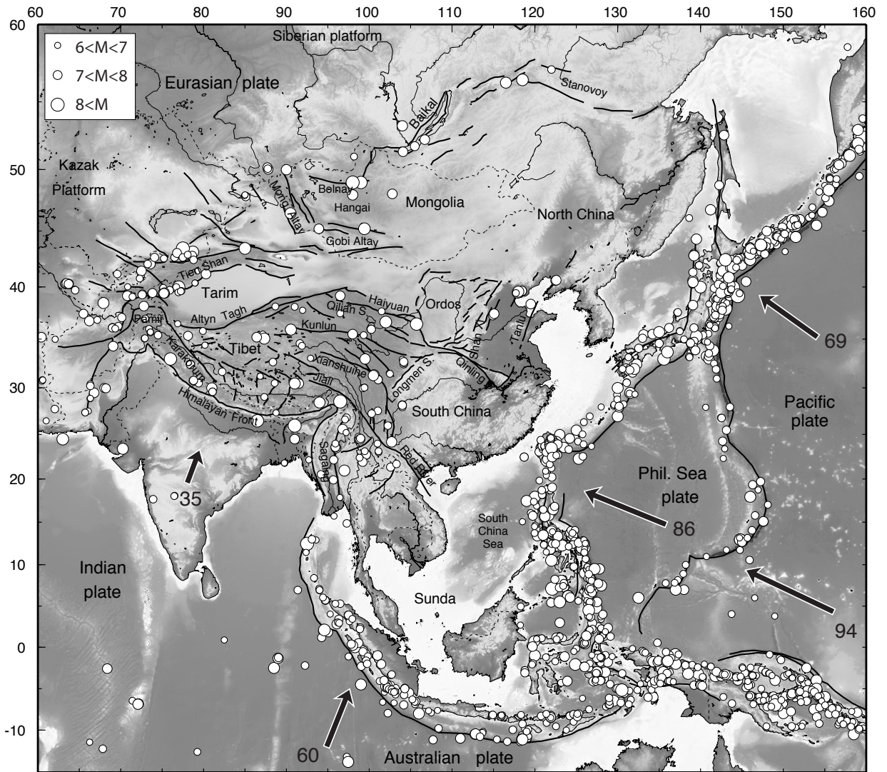
Figure 1. Topography, main active faults (black lines), seismicity (NEIC catalog, 1973-Present, M > 6 , depth < 80 km), relative plate motions with respect to Eurasia ( Sella et al. [2002]; values at arrow tails are in mm/yr), and index of the geographical names used in this paper.
