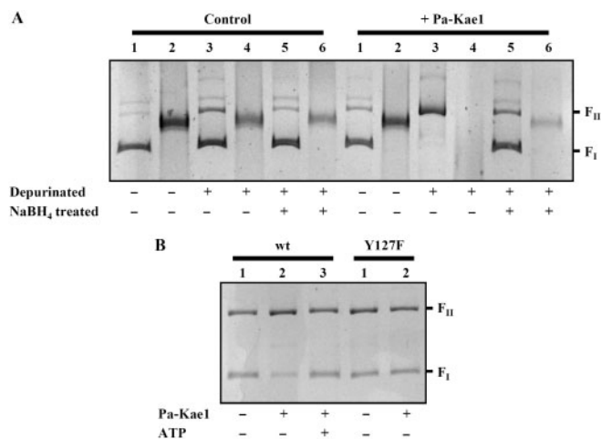
Figure 5. AP-endonuclease activity of Pa-Kael. (A) Detection of AP-endonuclease activity of Pa-Kael. AP-endonuclease activity was tested on untreated or depurinated DNA at 72°C for 10 min. Samples are then treated by SDS and Proteinase K to dissociate DNA/Pa-Kael complexes 30 min at 45°C and analysed by TAE-agarose gel electrophoresis. (1) untreated pBR322 DNA, (2) untreated \Phi X174 DNA, (3) depurinated pBR322 DNA, (4) depurinated \Phi X174 DNA, (5) depurinated pBR322 DNA treated by NaBH_4 , (6) depurinated \Phi X174 DNA treated by NaBH_4 incubated with or without Pa-Kael at a molar ratio of 1 protein for 2 nt (or base pairs). (B) Effect of the Y127F mutation on Pa-Kael activity. Depurinated pBR322 (1) was incubated with wild-type Pa-Kael and Y127 mutant as indicated in absence (2) or in presence (3) of ATP 10 mM for 10 min at 72°C. Products are then treated by SDS and Proteinase K for 30 min at 45°C and analysed by TAE-agarose gel electrophoresis.
