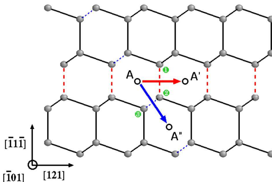
Figure 2. (color online) Ball-and-stick representation of the zinc-blende structure ( (\bar{1}01) plane). The path D' (D'') is defined by a dislocation displacement from A to A' (A to A''). Dashed lines show bonds linking atoms used for calculating the disregistry due to the dislocation core. In particular, atoms located in dislocation cores for saddle configurations are marked by numbers (1 and 2 for D', and 2 and 3 for D'').
