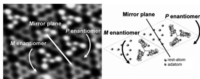
Figure 3. A room-temperature STM image ( V_s = -2.1 V, 7 \times 9 nm 2 ) showing the two enantiomers of the chiral supramolecular self-assembly of MSPS deposited on \text{Si}(111)-7 \times 7 (left) and a schematic model of these two enantiomers on \text{Si}(111)-7 \times 7 (right).
