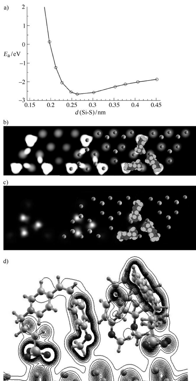
Figure 2. a) Adsorption energy as a function of distance. b,c) Integrated LDOS images of three MSPS molecules on \text{Si}(111)-7 \times 7 (left) and with a superimposed ball model (right) with a negative bias voltage (-2 V, b) and a positive bias voltage (+2 V, c). d) A side view of the density of states of MSPS adsorbed on \text{Si}(111)-7 \times 7 showing weak molecule-substrate interactions.
