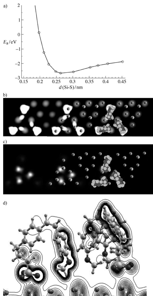
Figure 2. a) Adsorption energy as a function of distance. b,c) Integrated LDOS images of three MSPS molecules on Si(111)-7 \times 7 (left) and with a superimposed ball model (right) with a negative bias voltage (-2 V, b) and a positive bias voltage (+2 V, c). d) A side view of the density of states of MSPS adsorbed on Si(111)-7 \times 7 showing weak molecule-substrate interactions.
