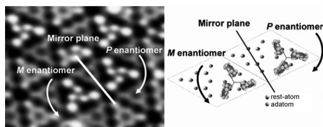
Figure 3. A room-temperature STM image ( V_s = -2.1 V, 7 \times 9 nm 2 ) showing the two enantiomers of the chiral supramolecular self-assembly of MSPS deposited on Si(111)-7 \times 7 (left) and a schematic model of these two enantiomers on Si(111)-7 \times 7 (right).
