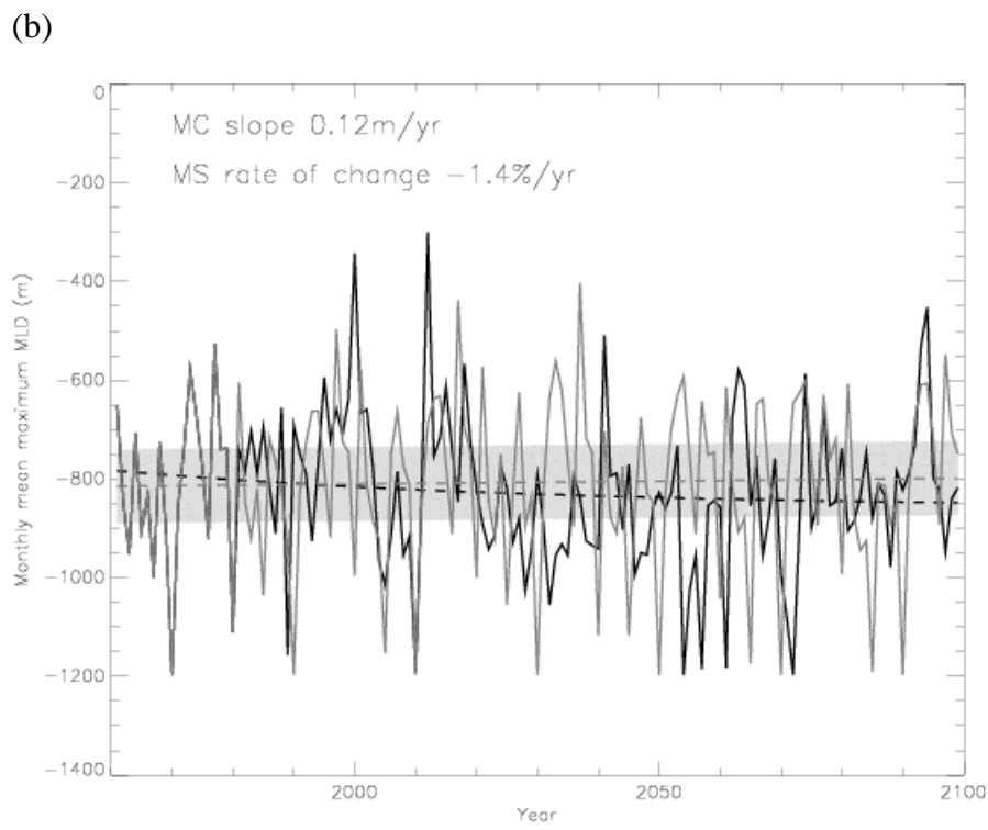
Fig 8: As for fig. 2, but for the maximum depth reached by the monthly mean mixed layer depth (1 point per year – in meters) (a) for the Levantine Basin, (b) for the Adriatic Sea, (c) for the Gulf of Lions area, and (d) for the Aegean Sea
