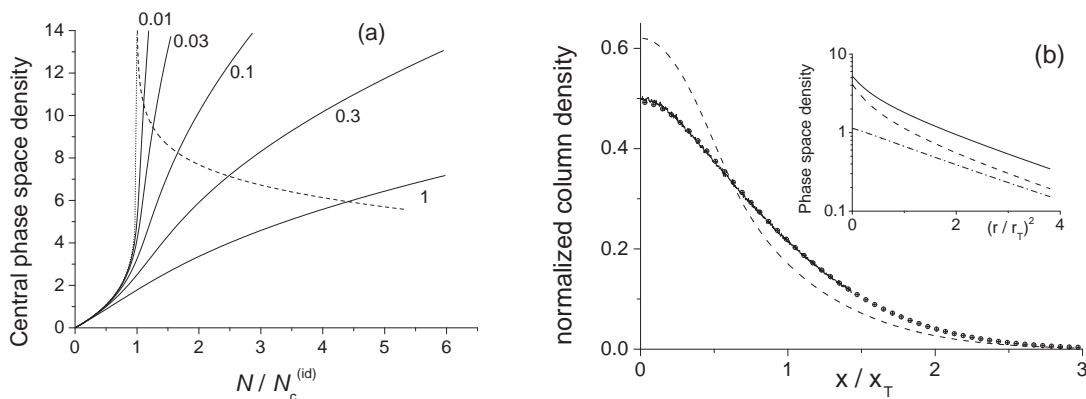
Figure 4. (a) Central phase space density predicted by the 2D mean field theory, as a function of the atom number for various interaction strengths \tilde{g} . The dotted line represents the semi-classical prediction for the ideal gas. The dashed line indicates where the threshold for superfluidity (11) is met at the center of the trap. (b) Column density for N = N_c^{(mf)} = 36\,000 atoms in an isotropic trap ( \omega_x = \omega_y = \omega , \tilde{g} = 0.13 , k_B T = 110\omega ). The dashed line is the result of the 2D mean-field analysis of § 4.3. The continuous line is the 3D quantum Monte-Carlo result obtained in [24], with \omega_z = 83\omega and a = \tilde{g}a_z/\sqrt{8\pi} . The dots are the result of the hybrid 3D mean-field calculation of § 4.5 for the same parameters. Inset: Prediction of the hybrid 3D mean-field approach for the phase space density (log scale) as a function of r^2 (a gaussian distribution leads to a straight line). Continuous line: total phase space density; dashed line: phase space density associated to the ground state \varphi_1 of the z motion; dash-dot line: phase space density associated to all other states \varphi_j, j \geq 2 .
