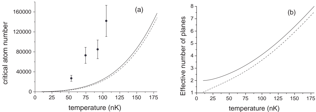
Figure 2. (a) Critical atom number N_c^{(\text{lat},\text{id})} in the ideal gas model for the optical lattice + magnetic trap configuration, as a function of temperature. The points represent the experimental results of [18], and the error bars combine the systematic and statistical uncertainties on atom numbers. (b) Effective number of planes \mathcal{N}_{\text{eff}} = N_c^{(\text{lat},\text{id})}/N_c^{(\text{id})} as a function of temperature. In both panels the continuous (dashed) line is for configuration A (B). The calculation is performed using the first 100 eigenvalues of the z motion, and the first neglected levels E_j(x) are 22 kHz ( 1 \mu\text{K} ) above the bottom of the trap.
