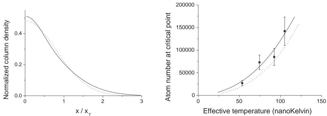
Figure 5. (a) Hybrid 3D mean-field prediction for the normalized column density for the lattice configuration A, T = 150 nK and N = 110\,000 atoms. For these parameters the phase space density associated to the lowest eigenvalue of the z motion reaches the critical value D_c at the center of the most populated planes. The dotted line is a gaussian fit which gives the effective temperature T_{\text{eff}} = 0.64 T = 96 nK. (b) Critical atom number as a function of the effective temperature obtained from a gaussian fit of the MF result. The continuous line (resp. dashed) line is for configuration A (resp. B). The points are the experimental results of [18], already shown in fig. 2.
