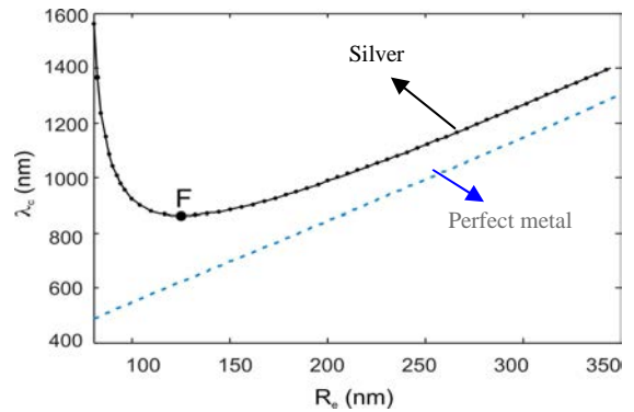
Fig.2: Modes of coaxial waveguide in silver, Mode TE_{11} , R_i=75\text{ nm} .
