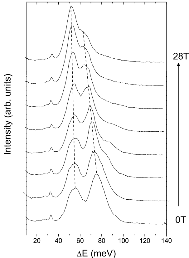
FIG. 2: Magneto-RPL spectra recorded on a p-doped sample at 4 K from B=0 to B=28 T every 4 T and for a E_{exc}=1260 meV. Traces have been vertically offset for clarity. The dashed lines are guides for the eyes.
