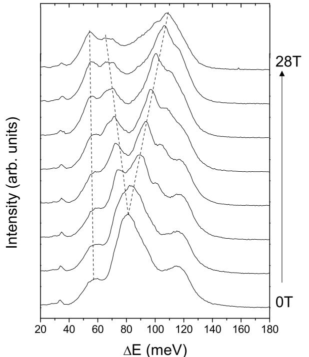
FIG. 1: Magneto-RPL spectra recorded on a p-doped sample at 4 K from B=0 to B=28 T every 4 T and for a E_{exc}=1293 meV. Traces have been vertically offset for clarity. The dashed lines are guides for the eyes.
