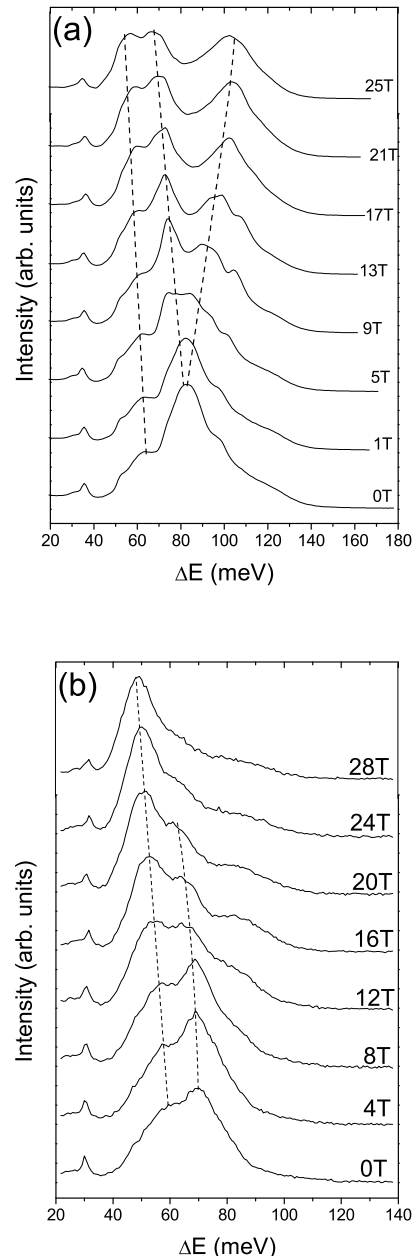
FIG. 3: Magneto-RPL spectra recorded on an undoped sample at 4 K from B = 0 to 25 T for E_{exc} = 1281 meV (a). Magneto-RPL spectra recorded on a n-doped sample at 4 K from B = 0 to 28 T for E_{exc} = 1259 meV (b). Traces have been vertically offset for clarity. The dashed lines are guides for the eyes.
