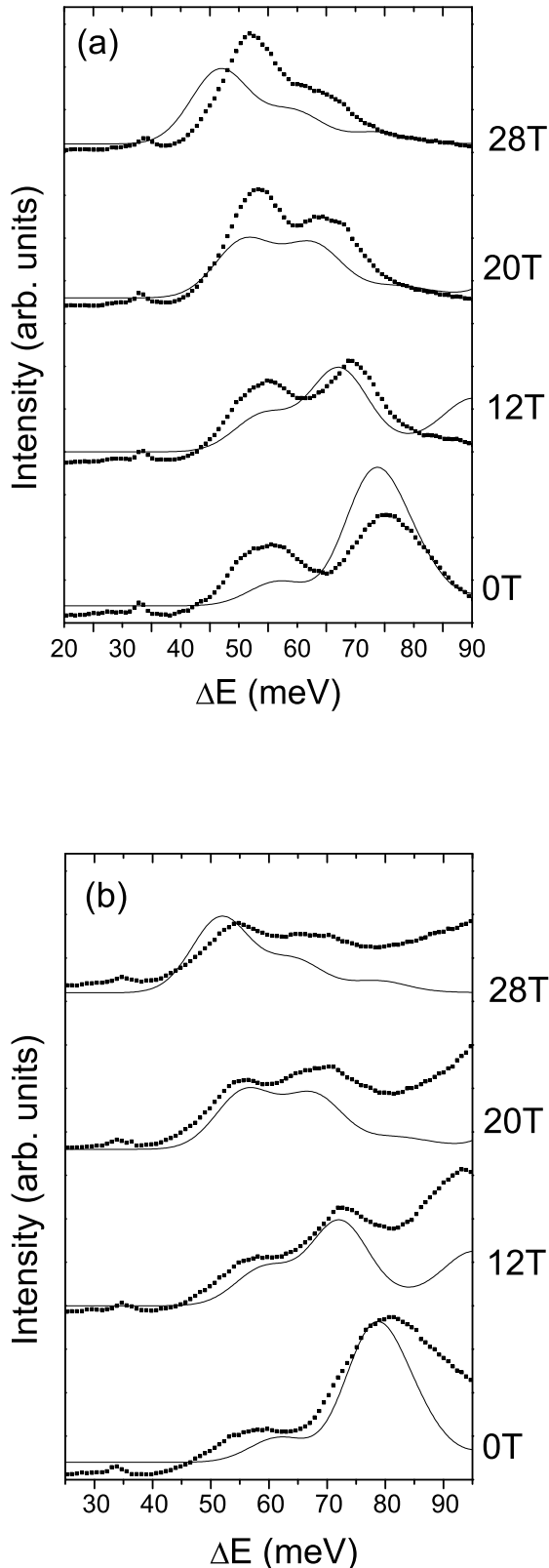
FIG. 6: Experimental (full symbols) and calculated (solid lines) spectra for different magnetic fields. The experimental data was taken for E_{exc}=1260 meV (a) and E_{exc}=1293 meV (b), for sample P3. The parameters used in the calculation are given in the text.
