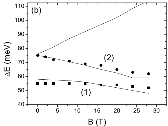
FIG. 5: Magnetic field dispersion of RPL resonances for E_{exc} = 1293 meV (a) and E_{exc} = 1260 meV (b) in symbols. The solid lines are the calculated polaron energy levels.
