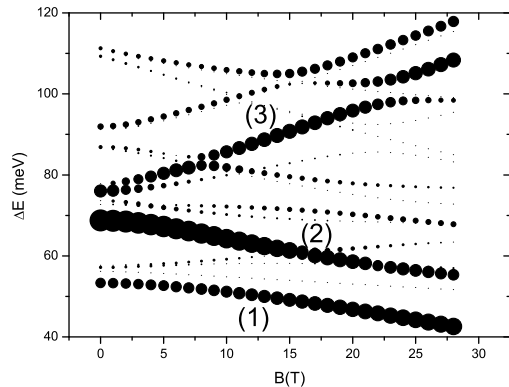
FIG. 4: Calculated excitonic polaron energies and intensities as a function of the magnetic field from reference 2. The area of the circles are proportional to the oscillator strengths.
