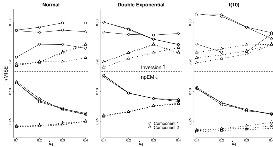
Figure 2: Square roots of Mean Integrated Squared Errors (MISE) are shown on a logarithmic scale as a function of \lambda_1 , the proportion of component 1, for three different simulated distributions for all f_{jk} , j = 1, 2 and k = 1, 2, 3 . The results for the inversion algorithm of Hall et al. (2005) are approximated from their plots on page 675, Fig. 2, with a small bit of noise added to separate coincident points.
