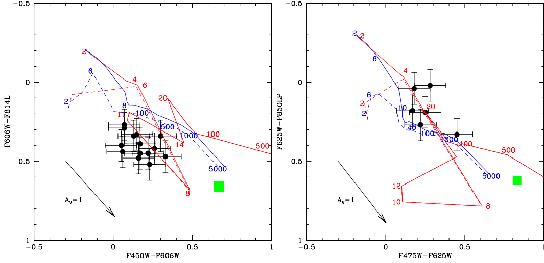
Figure 9. Colour–colour diagram for the blue knots in Abell 2667 (left) and Abell 1689 (right). The black circles with their associated error bars represent the knot colours and their uncertainties. The green squares indicate the colours of the two disrupted galaxies. The dashed lines are the model predictions for the evolution of simple stellar populations (SSPs) (red) and continuous (blue) star formation accounting for the contribution of emission lines. The solid lines represent the same models without the contribution of emission lines. The numbers indicate the age of each model in Myr. The black arrows show the effect of internal extinction on the observed colours. This figure is in colour in the online version of the article on Synergy .
