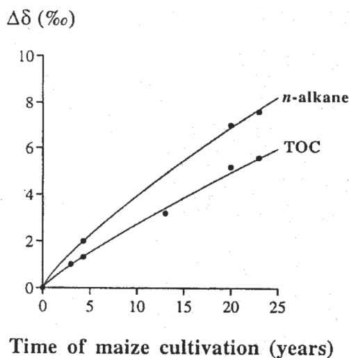
Figure 1. Isotope variations of total organic carbon (TOC) and of n -hentriacontane ( C_{31} ) from soils cultivated with Zea mays (see also Table 1). Note the faster increase of the individual n -alkane isotope variations.
