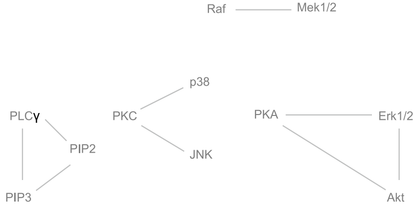
Figure 5: Graph \mathcal{G}_2
