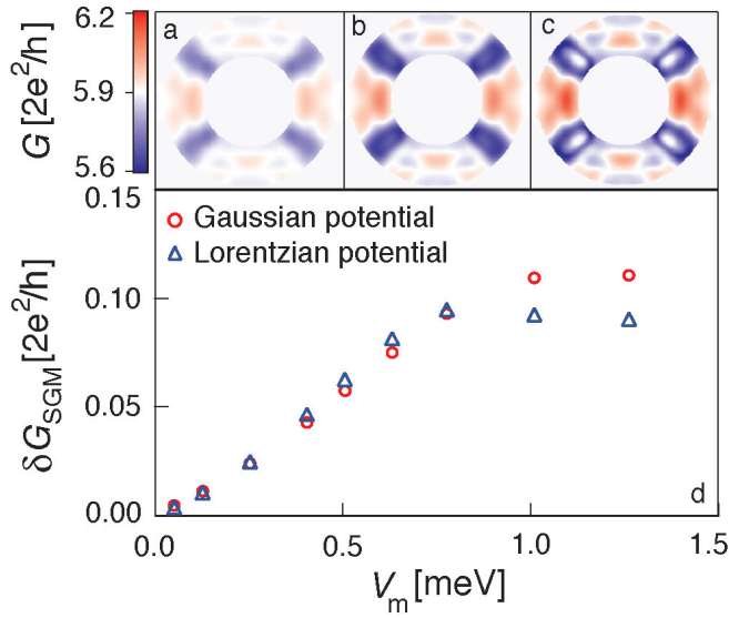
FIG. 4: (Color online) (a-c) Simulated G maps, calculated for E_F = 101 meV, \sigma = 20 nm and V_m = 0.5, 1.0 and 1.5 meV, respectively. (d) Fringe amplitude \delta G_{SGM} on simulated G maps as a function of V_m , with \sigma = 20 nm.
