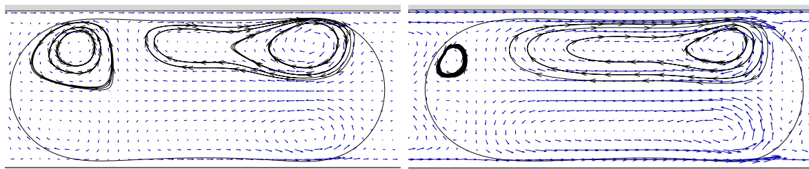
Figure 2. Various regimes for a confined droplet in a microchannel (wall in grey, velocity field in blue, interface in black and some streamlines in arrowed-line) : on the left, injection velocity is lower than on the right.
