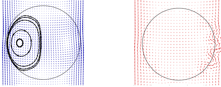
Figure 1. on the left (velocity field in blue, interface in black and some streamlines in arrowed-line), c_2 = 8 and the computation is stable for a medium grid, whereas on the right (velocity field in red, interface in black), c_2 = 9 and the instability appears on the same grid ; velocity fields are those in the drop frame of reference
