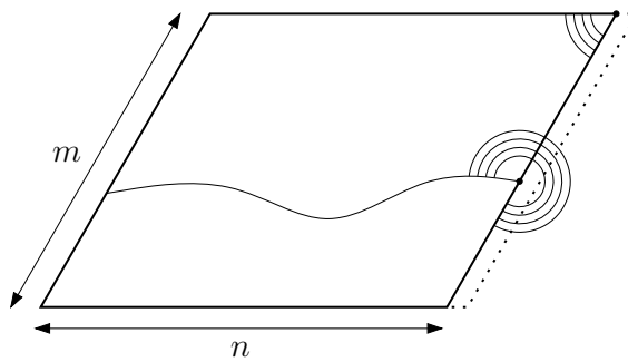
Figure 15: We extend a crossing of [0, n] \times [0, m] into a crossing of [0, (1 + \eta)n] \times [0, m] by applying RSW in concentric annuli.
