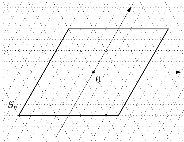
Figure 2: We refer to oblique coordinates, and we denote by S_n the “box of size n ”.
