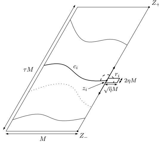
Figure 6: Well-separateness for a set of crossings \mathcal{C} = \{c_i\} .
