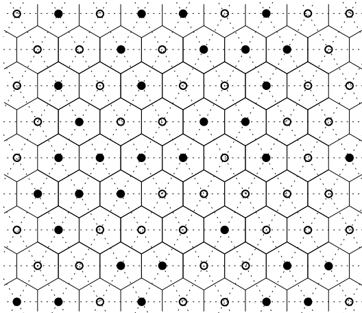
Figure 1: Percolation on the triangular lattice can be viewed as a random coloring of the dual hexagonal lattice.
