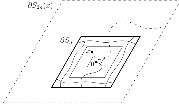
Figure 18: With this construction, any site x in S_{n/3, 2n/3} connected to a site at distance 2n is also connected to 0 in S_n .
