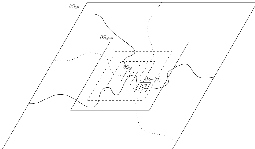
Figure 11: If v is pivotal, 4 alternating arms arise locally.
