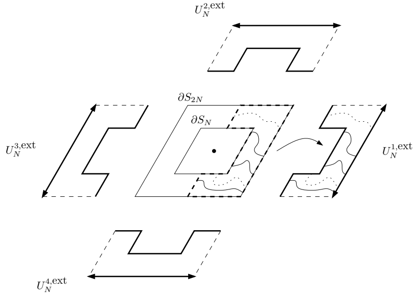
Figure 7: The four U-shaped regions that we use for the external extremities.
