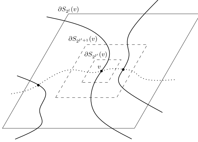
Figure 12: More complex events may arise when \sigma is not alternating.
