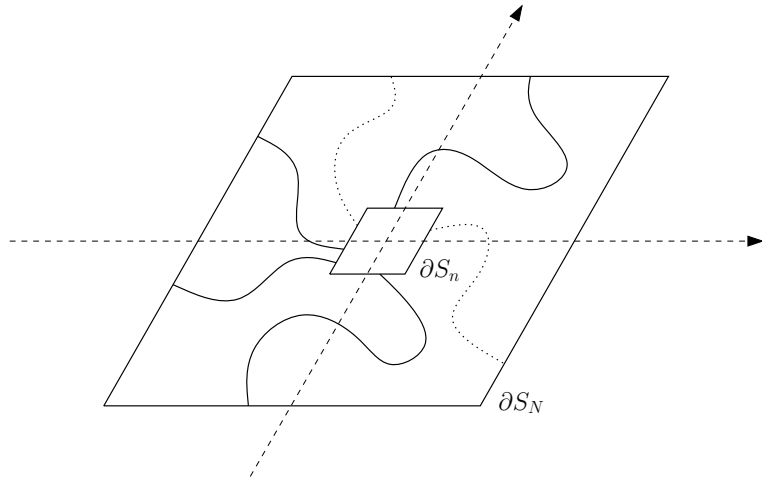
Figure 5: The event A_{6,\sigma}(n, N) , with \sigma = BBBWBW .
