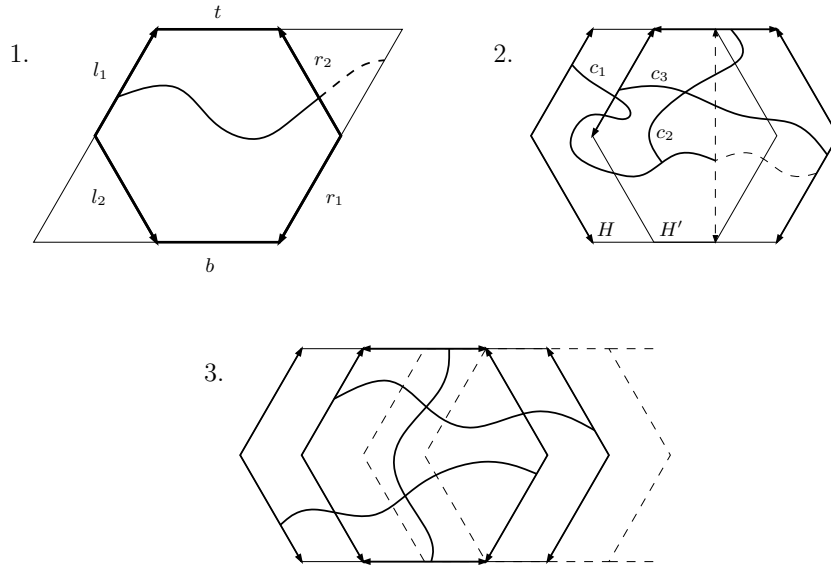
Figure 4: Proof of the RSW theorem on the triangular lattice.
