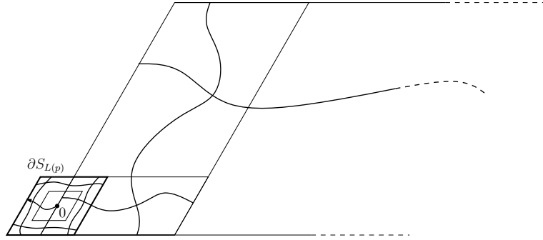
Figure 17: We consider overlapping parallelograms, with size doubling at each step.
