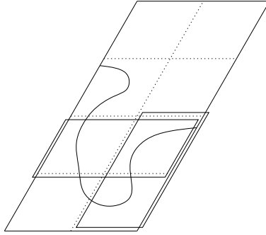
Figure 16: Two of the small sub-parallelograms are crossed in the “easy” way.
