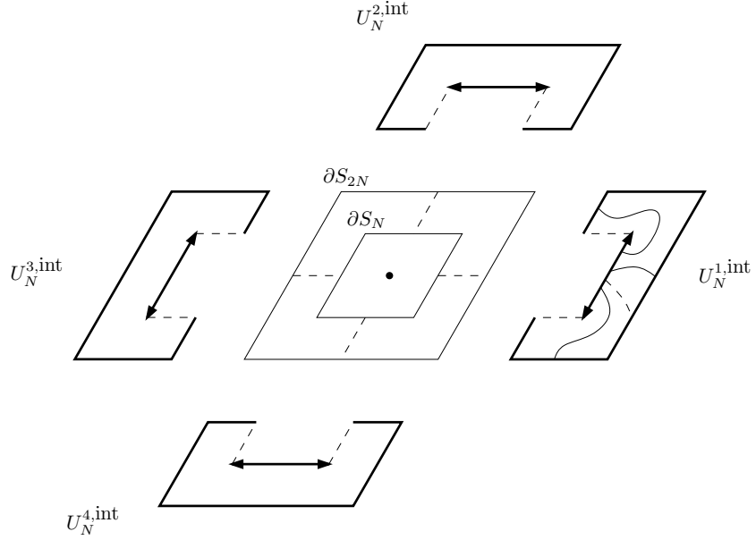
Figure 9: For the internal extremities, we consider the same domains but we mark different parts of the boundary.
