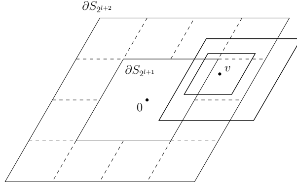
Figure 13: We replace R(v) = S_{2^l}(v) by one of the R_{2^{l+1}}^i ( i = 1, \dots, 12 ).
