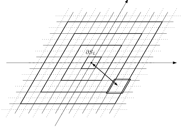
Figure 19: For the upper bound, we cover the plane with rhombi of size 2L and sum their different contributions.
