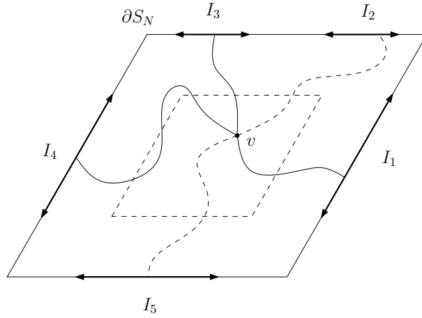
Figure 10: The landing sequence I_1, \dots, I_5 .
