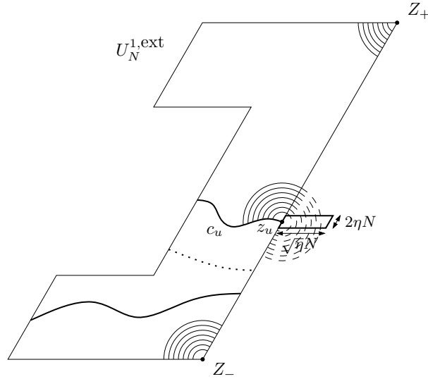
Figure 8: We apply RSW in concentric annuli around Z_- and Z_+ , and then around the extremity z_u of each crossing c_u .
