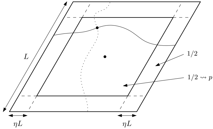
Figure 14: We restrict to the sites at distance at least \eta L from the boundary of [0, L]^2 : these sites produce contributions of the same order, since the 4 arms stay comparable in size.
