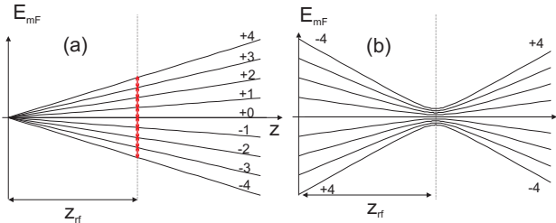
Fig. 4 Modification of the magnetic potential in presence of a strong rf field with frequency \omega_{rf}/2\pi . (a) Initial potentials with B(0, 0, z) = b'.z . (b) The magnetic potentials are distorted into nine adiabatic potentials. The coupling takes place at the isoB plane position Z_{rf} = \hbar\omega_{rf}/g_F\mu_B b' . At this position the energy separation between the different adiabatic potentials is of the order of \hbar\Omega
