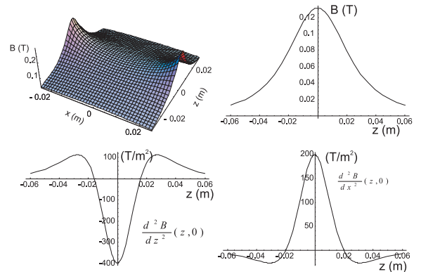
Fig. 2 Space dependence of the magnetic field amplitude and its second derivatives. The magnetic field amplitude is plotted for a current in the coil of 100 A.
