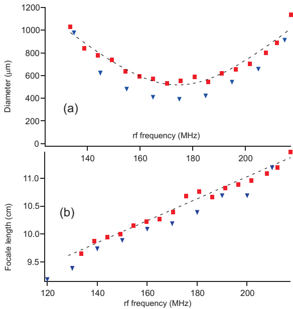
Fig. 6 (a) Variation of the cloud diameter at the probe position as a function of the rf frequency. The current in the coil is 85 A. (b) Corresponding variation of the focal length with the rf frequency. The experimental data are deduced from (a) (see text). For (a) and (b) : Experiment (squares) , numerical simulation (triangles). The dashed lines are guides for the eye.
