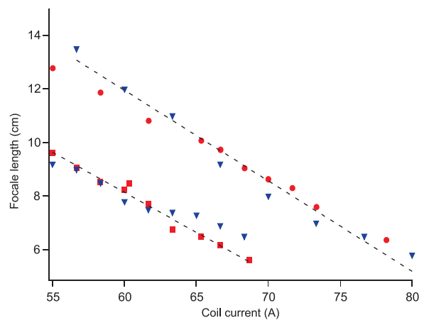
Fig. 7 Evidence for a rf-induced increase in the lens power. The focal length is plotted versus the coil current for configuration 2. The rf frequency is set to 210 MHz. Experimental data (squares) = with rf, (circles) = no rf, and numerical calculations (triangles). The dashed lines are guides for the eye. (The increase of the focusing power of the lens with the rf is evident from a comparison of the two sets of points.)
