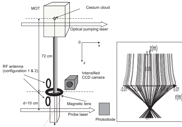
Fig. 1 Schematic of the experimental set-up. The lens is made of a vertical axis coil, centered about 72 cm below the MOT center. The rf antenna is located a few cm above (configuration 1) or below (configuration 2) the lens center, with its axis along the Ox direction. The inset on the right shows 100 atomic trajectories as the cloud crosses the magnetic lens plane.
