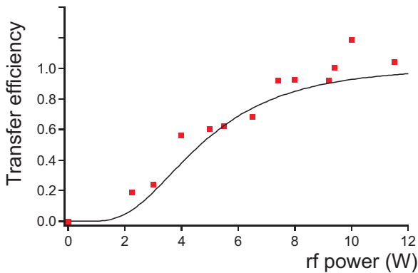
Fig. 8 Transfer efficiency as a function of the rf power. The rf frequency was fixed to 130 MHz, the current in the lens to 95 A. Atoms are initially polarized in |m_F = -4\rangle state (configuration 1) and we measure the number of atoms focused at the probe position and normalized it (see text). The black line is obtained from 5, the scaling between \Omega^2 and the rf power being given by the experimental calibration.
