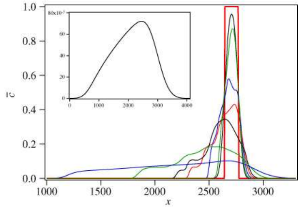
FIG. 3: Transverse average profiles of concentration at successive times t=0 , 500, 700, 1000, 1500, 2000, 5000 and 15000. Inset: transverse average profile of concentration at t = 60000 ( Pe = 512 , l = 128 , R = 2 , \varepsilon = 1 ).
