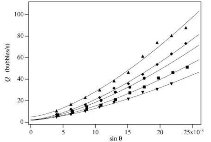
FIG. 4: Bubble flow rate Q as a function of the tilt angle \theta of the plane. The curves correspond to different apertures D of the silo: ( \blacktriangledown ) D = 6.3 mm, ( \blacksquare ) D = 8.0 mm, ( \bullet ) D = 9.7 mm, ( \blacklozenge ) D = 12.8 mm, ( \blacktriangle ) D = 19.9 mm; (—) best fit of the experimental data with Q \propto (\sin \theta)^{3/2} .
