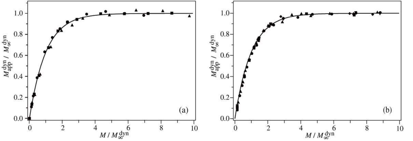
FIG. 3: Reduced apparent mass M_{\text{app}}^{\text{dyn}}/M_{\infty}^{\text{dyn}} vs. reduced total mass M/M_{\infty}^{\text{dyn}} (bead diameter d = 2 \text{ mm} ). The solid line corresponds to Eq. (3) — (a) Tube velocity: V = 4 \text{ mm s}^{-1} , relative humidity: (●) H = 25\% , (■) H = 60\% , (▲) H = 80\% . — (b) Relative humidity: H = 60\% , tube velocity: (◆) V = 0.02 \text{ mm s}^{-1} , (■) V = 0.2 \text{ mm s}^{-1} , (●) V = 2 \text{ mm s}^{-1} , (▲) V = 20 \text{ mm s}^{-1} , (▼) V = 34 \text{ mm s}^{-1} .
