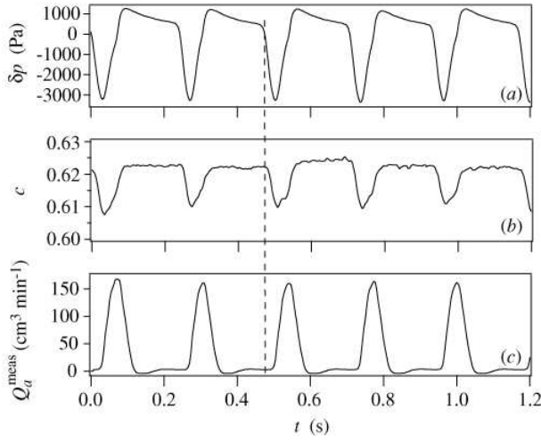
FIG. 10: Time recordings of the pressure deviations \delta p and particle fraction c variations (at z = 200 mm) and of the measured air flow-rate Q_a^{\text{meas}} into the hopper. Q_a^{\text{meas}} is defined as positive for air flowing downwards. The dashed line corresponds to the onset of the flow.
