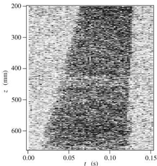
FIG. 7: Processed spatio-temporal diagram over a 500 mm length of tube ( 200 \text{ mm} < z < 700 \text{ mm} ) during one period of the intermittent flow. Light zones correspond to the static phase and the darker region to the flow.
