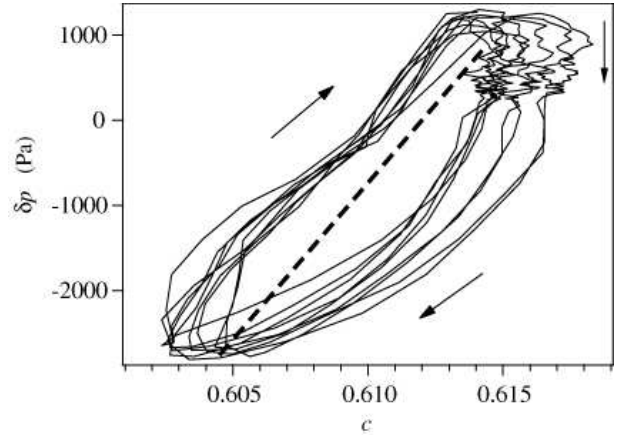
FIG. 12: Pressure vs. particle fraction variations during 10 cycles of the intermittent flow. Arrows indicate the direction of the variation on each part of the curve: the vertical phase corresponds to the slow pressure relaxation through the motionless grain packing, the lower section corresponds to the onset of the flow and the upper one to the blockage of the flow. The dashed line has the theoretical slope \gamma p_o/(1 - \overline{c}) .
