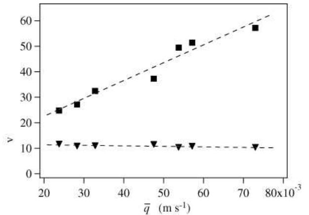
FIG. 8: Variation of the absolute velocities of propagation of the decompaction |v_{df}| (▼) and blockage |v_{bf}| (■) fronts with the mean superficial grain velocity \bar{q} .
