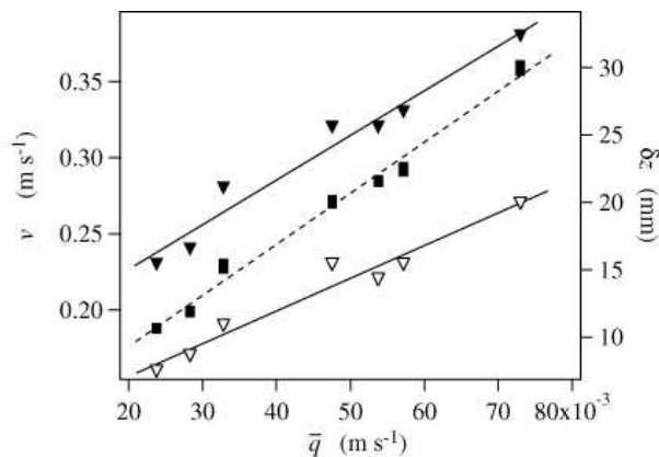
FIG. 4: Mean grain velocity \bar{v} vs. mean superficial velocity \bar{q} for z = 250 mm (▼, left axis) and z = 600 mm (▽, left axis). Displacement \delta z of the grains during a flow period as a function of \bar{q} (■, right axis).
