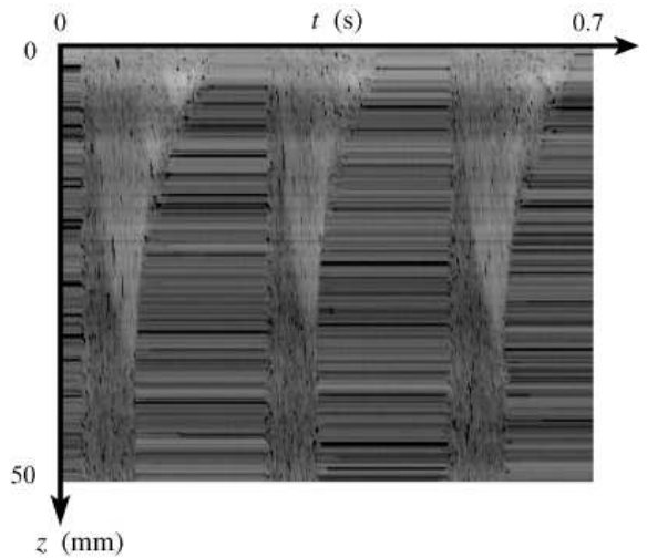
FIG. 5: Spatio-temporal diagram of the grain flow at distances between 0 mm and 50 mm from the hopper at the top of the tube ( \bar{q} = 0.07 m s ^{-1} ); total time lapse corresponding to diagram: 0.7 s.
