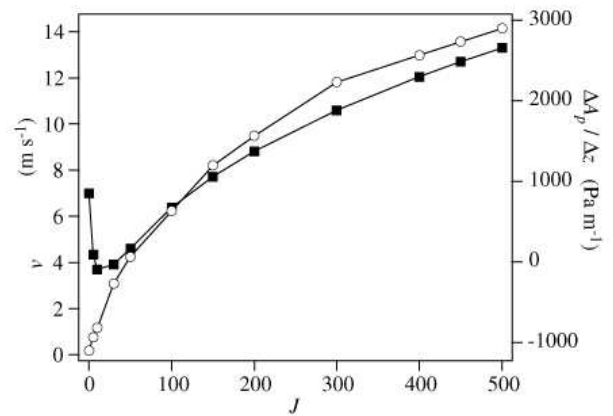
FIG. 14: Variation of the amplification parameter \Delta A_p/\Delta z (○) and of the absolute front velocity |v_{bf}| (■) with the force parameter J , for K = 20 \cdot 10^{-12} \text{ m}^2 .
