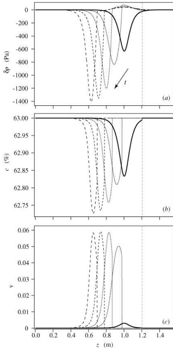
FIG. 13: Numerical pressure (a), particle fraction (b) and velocity (c) profiles, obtained for J = 450 , K = 20 \cdot 10^{-12} \text{ m}^2 and c_{max} = 0.63 . From right to left: solid lines: initial profile at t = 0 \text{ s} - dashed lines: t = 9 \text{ ms} , t = 15 \text{ ms} , t = 21 \text{ ms} , t = 27 \text{ ms} (dash length and spacing increases with time). The vertical dashed lines represents the position of the front z_f at t = 0 \text{ s} .
