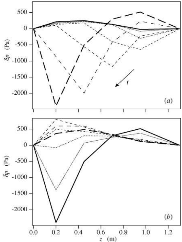
FIG. 9: Pressure deviation ( \delta p = p - p_o ) variations with distance along the tube for several measurement times, for a mean superficial velocity \bar{q} = 0.02 \text{ m s}^{-1} . (a) Solid line obtained during the static phase at t = 0 \text{ s} . Dashed lines are profiles obtained at various times during the flowing phase: t = 16 \text{ ms} , t = 31 \text{ ms} , t = 62 \text{ ms} , t = 86 \text{ ms} , t = 109 \text{ ms} and t = 133 \text{ ms} (dash length and spacing increase with time). (b) Solid line obtained near the end of the flowing phase at t = 133 \text{ ms} . Dashed lines are profiles obtained at various times: t = 141 \text{ ms} , t = 148 \text{ ms} , t = 156 \text{ ms} , t = 172 \text{ ms} , t = 211 \text{ ms} , t = 266 \text{ ms} (dash length and spacing increase with time).
