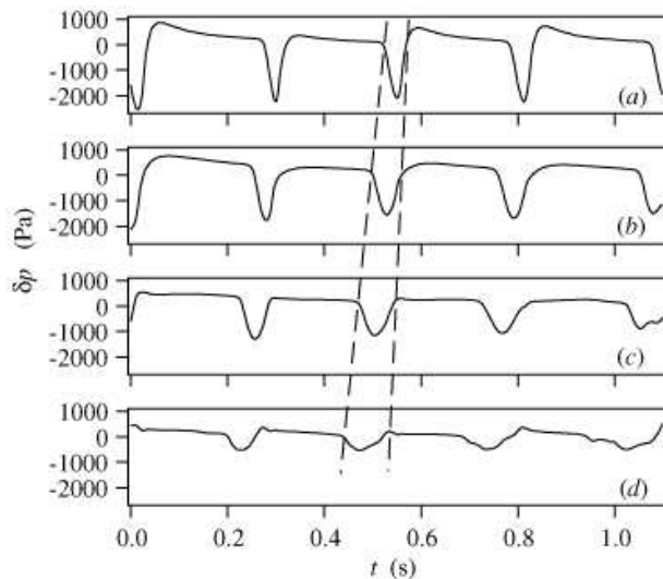
FIG. 6: Time recording of pressure variations \delta p at four different distances z from hopper (from top to bottom, z = 200, 450, 700 and 950 mm), for \bar{q} = 0.02 \text{ m s}^{-1} . Dashed lines correspond to the onset and the blockage of the flow.
