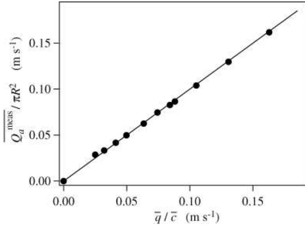
FIG. 11: Average inflow of air as a function of \overline{q}/\overline{c} .
