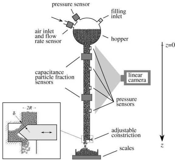
FIG. 1: View of the flow experiment. - Insert: sketch of the constriction at the bottom end of the pipe.
