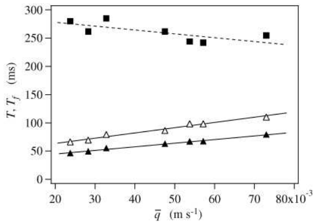
FIG. 3: Duration of flow phase T_f , as a function of the time average \bar{q} of the superficial velocity, at two different distances z from the top of the tube: z = 250 mm (▲) and z = 600 mm (△). Global period of the intermittent flow T (■).
