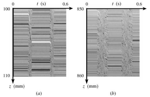
FIG. 2: Spatio-temporal diagram of the grain flow: (a) at the top of the tube (100 mm to 110 mm from the hopper), (b) at the bottom of the tube (850 mm to 860 mm from the hopper). Each diagram corresponds to a time lapse of 0.6 s and to a field of view of 10 mm.
