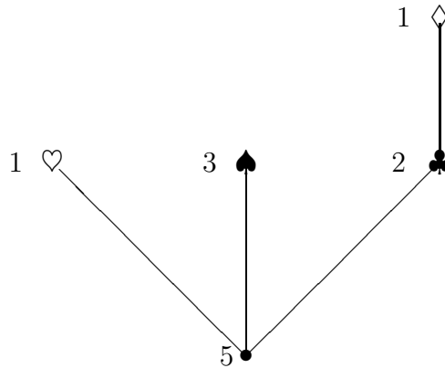
Figure 2 : Allelic tree corresponding to the genealogical tree with mutations in Figure 1. The labels represent the sizes of the allelic clusters.
