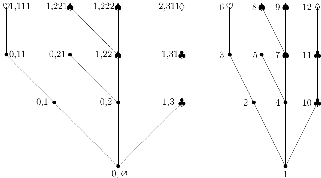
Figure 1 : Depth-first search with mutations on a genealogical tree. The symbols \bullet, \spadesuit, \heartsuit, \diamond, \clubsuit represent the different alleles. Left : The label (m, s) of an individual is given by the number m of mutations and the sequence s that specifies its genealogy; for the sake of
