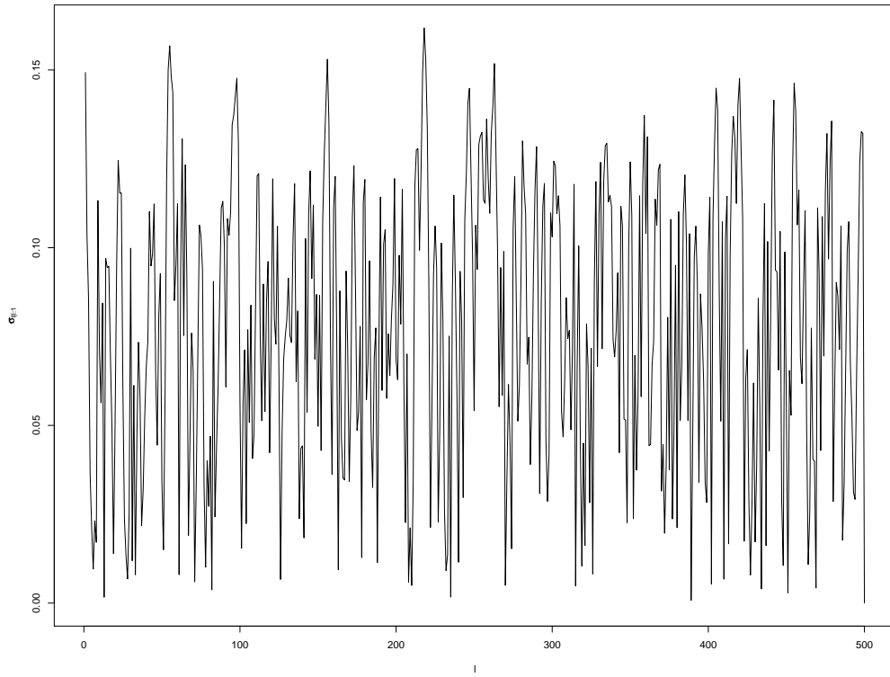
Figure 3. Evolution of the scale parameter \sigma_{l|l:1} of the conditional distribution \mathcal{L}(X_l|Y_l, \dots, Y_1) as l increases. The hidden process (X_n) is specified to be ergodic.
