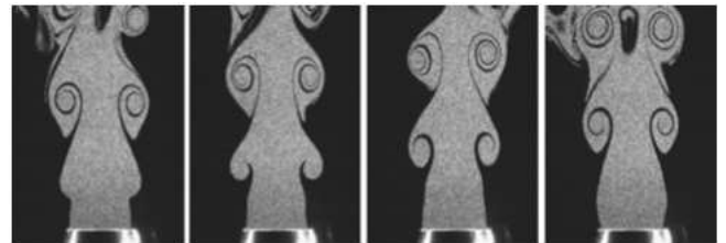
Figure 1: Tomographic images of an excited jet. Flow exit velocity on the axis: 2.5 \text{ m.s}^{-1} , diameter: 22 mm, frequency: 46 Hz. St = 0.41 and Re = 3660 . Each image is shifted of \pi/2 (Birbaud et al. (2007))
