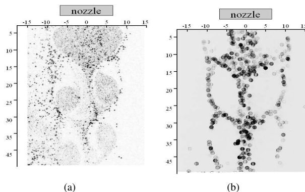
Figure 9: Instantaneous modulated air flow and decane spray. (a) Tomographic focused image of the air flow seeded with oil (light gray particles) and the decane spray (black dots). (b) Defocused image of the decane spray. Due to their small size, the oil droplets are not visible.
