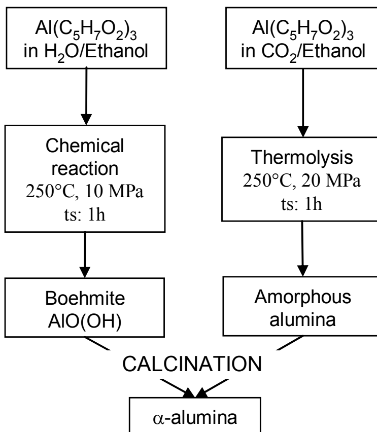
Fig. 1. Flow diagrams for the two routes used to produce \alpha -alumina in sub- and supercritical fluid media (ts : residence time, pc : critical pressure, Tc : critical temperature).
