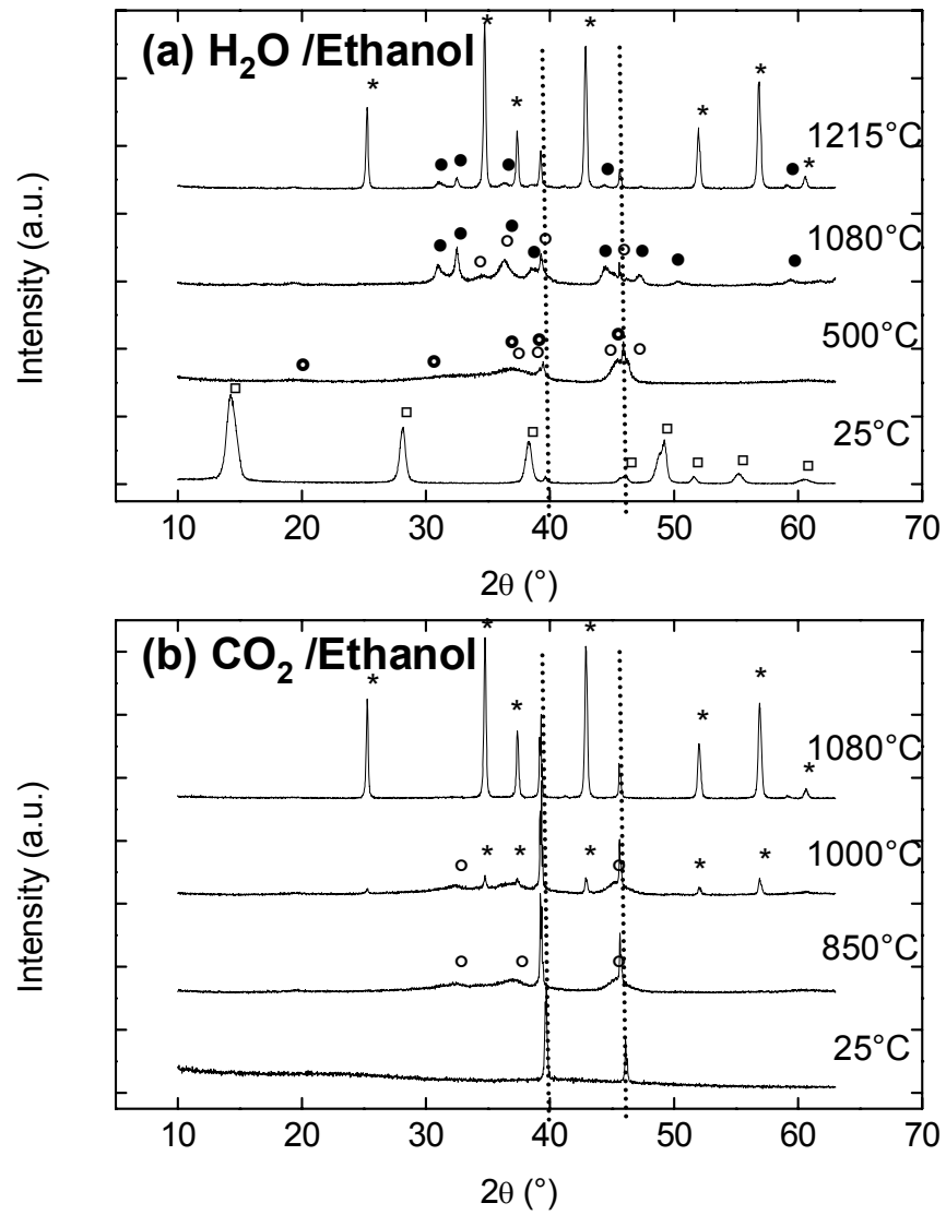
Fig. 4. Structural evolution with temperature of powders synthesized in (a) water/ethanol (□ boehmite, ○ \gamma -alumina, ● \delta -alumina, ● \theta -alumina and * \alpha -alumina) and (b) CO 2 /ethanol. (○ \gamma -alumina, * \alpha -alumina).
