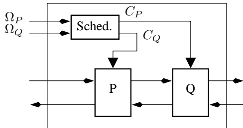
Figure 8. Quasi-synchronous activation
