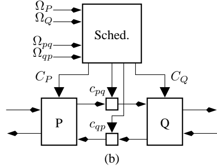
Figure 3. Modeling non synchronous executions
