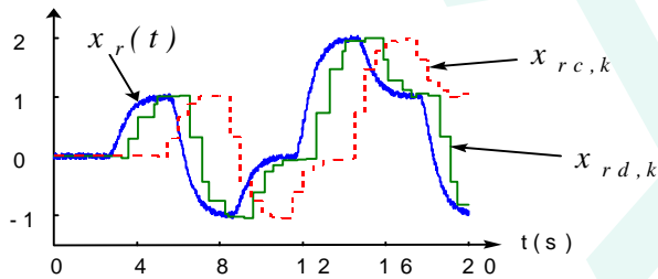
Figure 10 - Effects of the delay variation balancer
