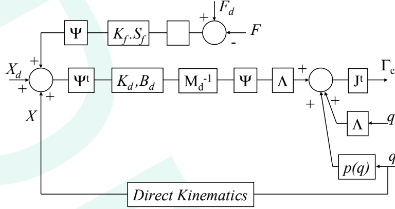
Figure 4: Impedance control scheme
