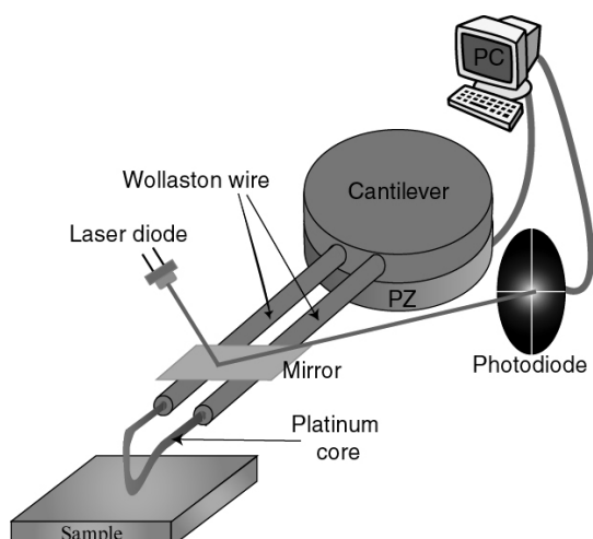
Figure 4: STHM schematic view
