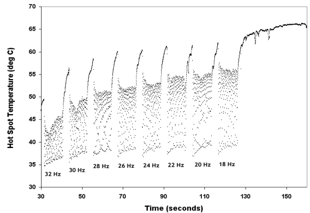
Figure 4. Variation in the temperature of the hot spot with the droplet shuttling at various frequencies. At each frequency, the droplet was shuttled back and forth the linear array for 10s, and stationarily held away from the hot spot for 5s to allow any heat stored in the droplet to dissipate. At the end of the experiment, the hot spot was allowed to reach a steady-state temperature.
