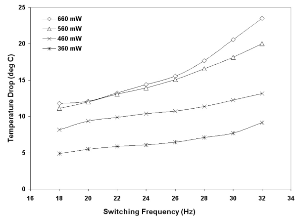
Figure 5. Temperature drop at the hot spot with respect to switching frequency of a shuttling droplet as a function of input power.
