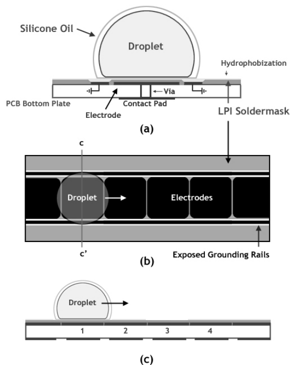
Figure 1. Schematic of a coplanar digital microfluidic chip on PCB. The side view (a) represents the cross section c-c' as specified in the top view (b). Droplet transport is shown from the side (c) and top (b) view of the electrowetting chip. A droplet is held onto electrode 1 by applying a voltage (240V) at that electrode. Droplet transport to the right is achieved by deactivating electrode 1 and activating electrode 2 simultaneously. This creates a reduction in interfacial tension on the leading edge of the droplet, causing the droplet to move until it is aligned onto the center of the new electrode.
