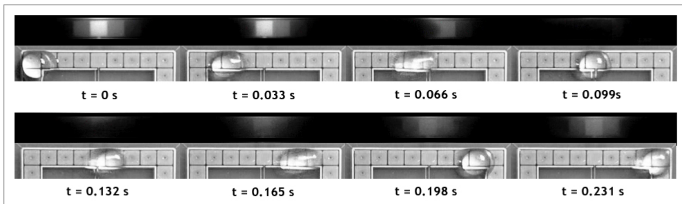
Figure 3. Top view of droplet transport as viewed from an infrared camera (top image in each frame, white = hot) and regular camera (bottom image). A droplet volume of volume 6 \mu l is transported across the hot spot (65°C) at a switching frequency of 32 Hz. The hot spot is cooled by 20°C at t = 0.231 s.
